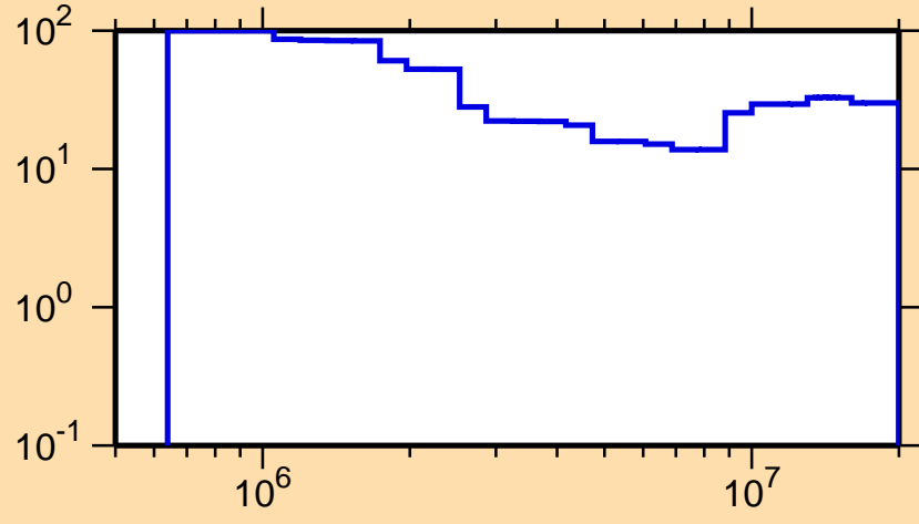
\Delta\sigma/\sigma vs. E for ^{187}\text{Au}(n,n\text{cont.})
