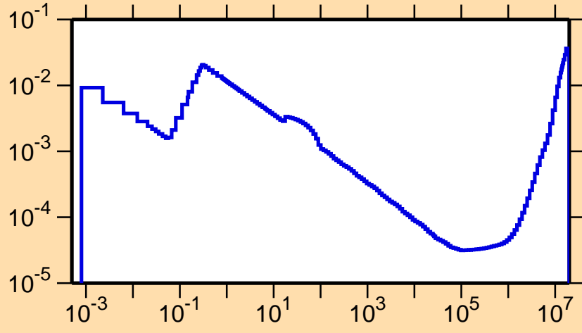
\sigma vs. E for ^{187}\text{Au}(n,\alpha)
