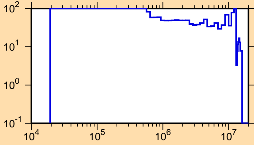
\Delta\sigma/\sigma vs. E for ^{187}\text{Au}(n,n_1)
