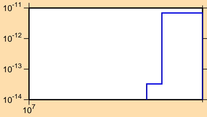
\sigma vs. E for ^{187}\text{Au}(n,\text{pt})
