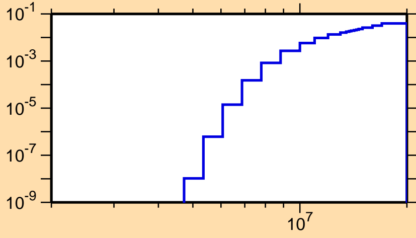
\sigma vs. E for ^{187}\text{Au}(n,np)
