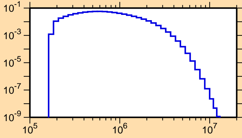
\sigma vs. E for ^{187}\text{Au}(n,n_3)
