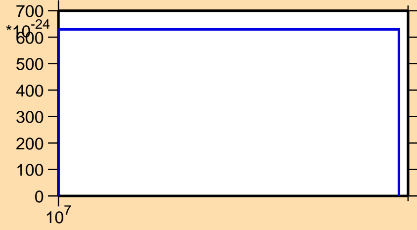
\sigma vs. E for ^{187}\text{Au} (mt 42)
