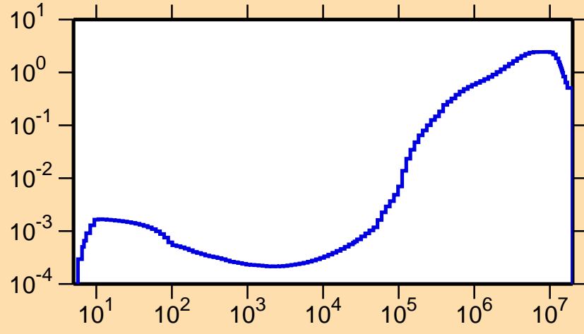
\sigma vs. E for ^{187}\text{Au}(n,\text{inel.})
