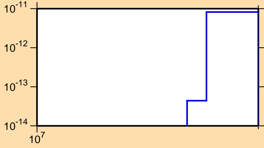
\sigma vs. E for ^{187}\text{Au}(n,pt)
