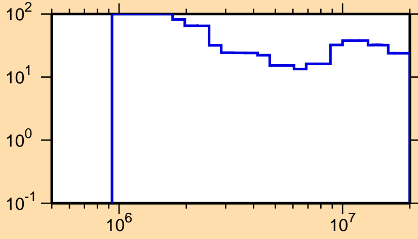
\Delta\sigma/\sigma vs. E for ^{188}\text{Au}(n,n\text{cont.})
