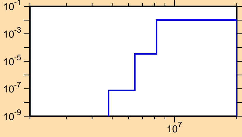
\sigma vs. E for ^{188}\text{Au}(n,np)
