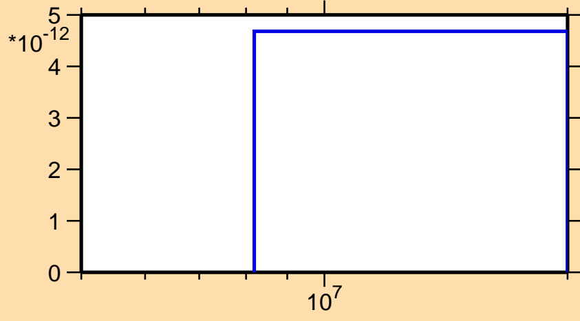
\sigma vs. E for ^{188}\text{Au}(n,pd)
