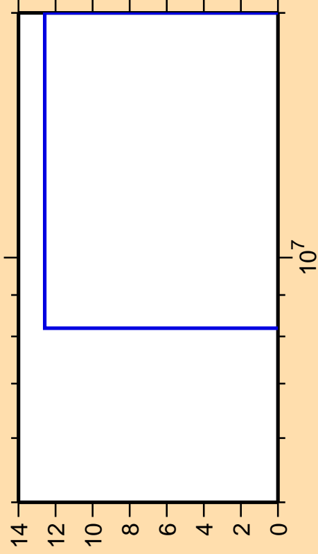
\Delta\sigma/\sigma vs. E for ^{188}\text{Au}(n,pt)
