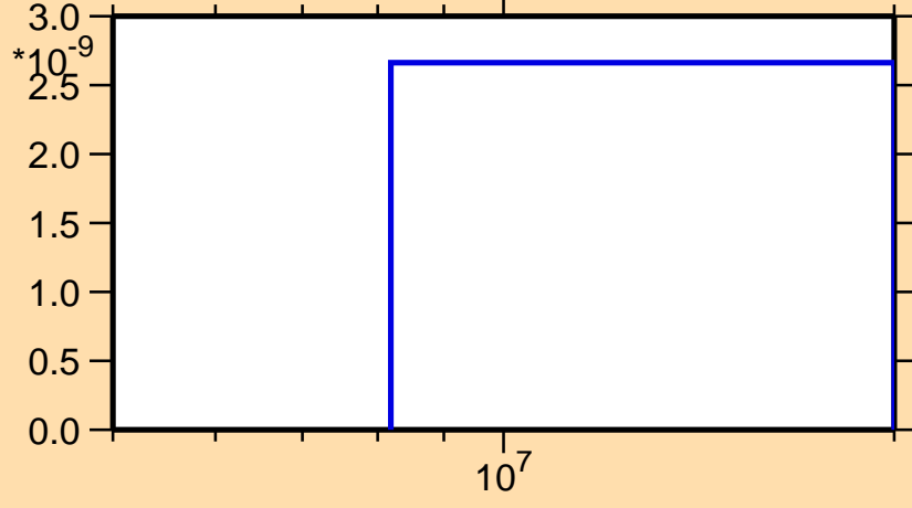
\sigma vs. E for ^{188}\text{Au}(n,nt)
