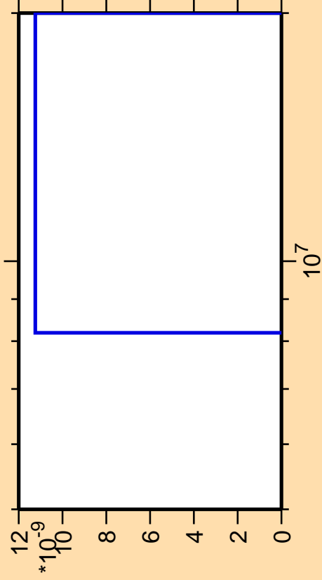
\Delta\sigma/\sigma vs. E for ^{188}\text{Au}(\text{mt } 42)
