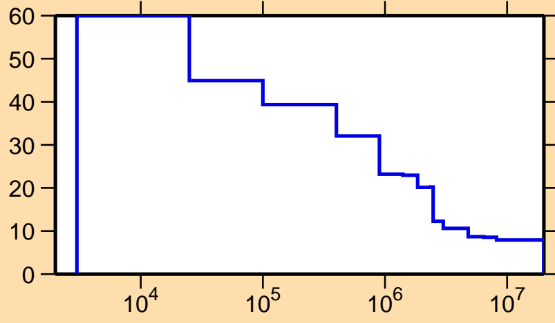
\Delta\sigma/\sigma vs. E for ^{188}\text{Au}(n,\text{nonel.})
