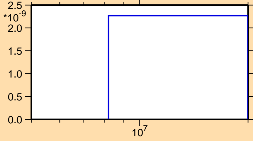
\sigma vs. E for ^{188}\text{Au}(\text{mt } 45)
