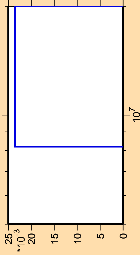
\Delta\sigma/\sigma vs. E for ^{188}\text{Au}(n,3n\alpha)
