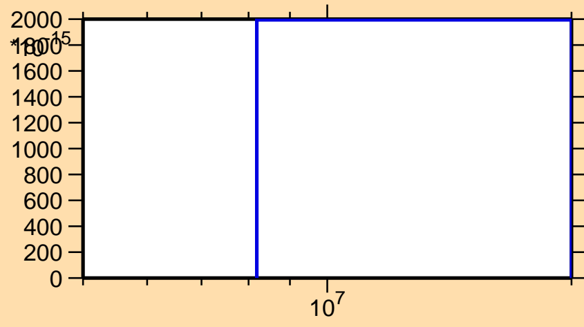
\sigma vs. E for ^{188}\text{Au}(n,pt)
