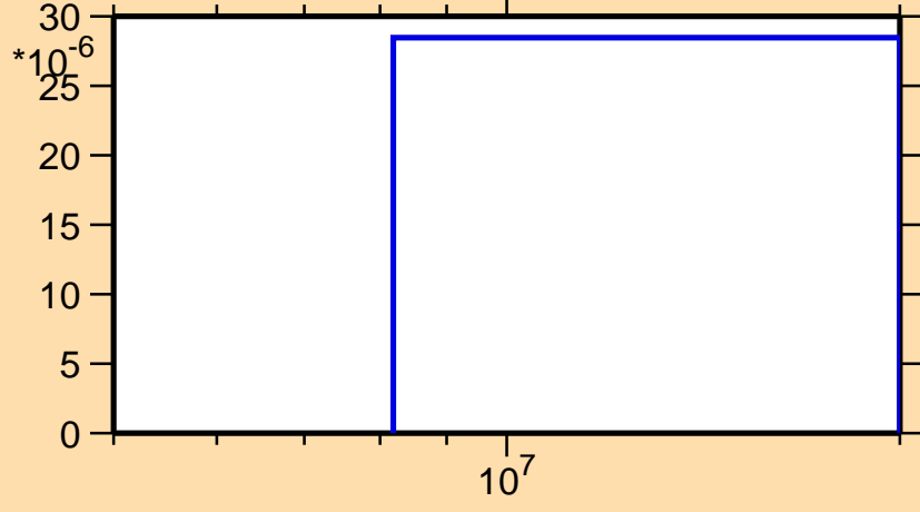
\sigma vs. E for ^{188}\text{Au}(n,2np)
