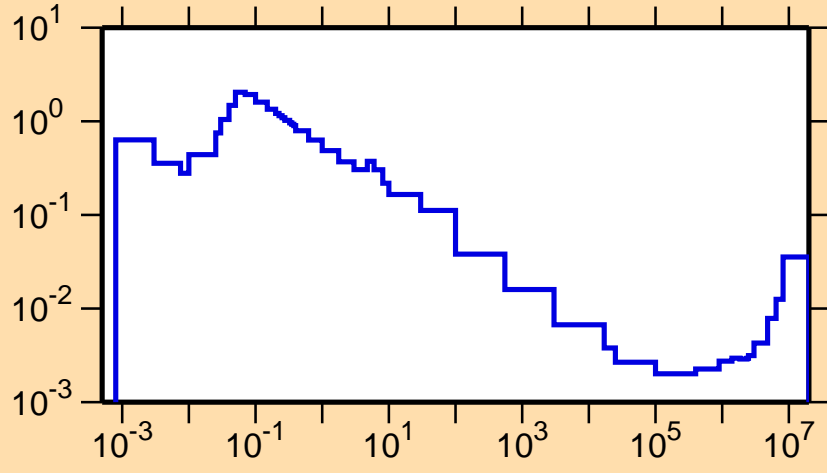
\sigma vs. E for ^{188}\text{Au}(n,p)
