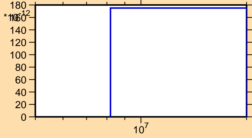
\sigma vs. E for ^{188}\text{Au}(\text{mt117})
