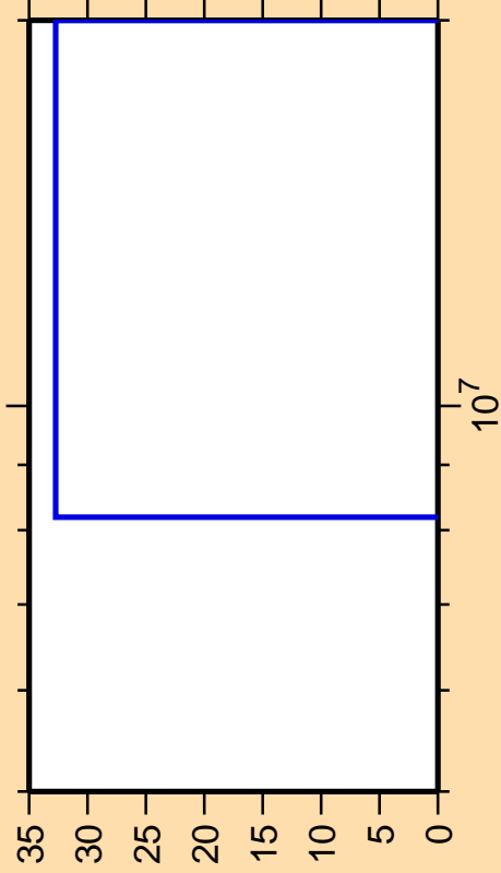
\Delta\sigma/\sigma vs. E for ^{188}\text{Au}(n,pd)
