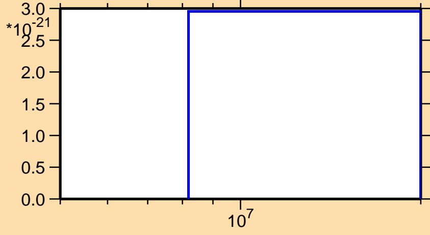
\sigma vs. E for ^{188}\text{Au}(\text{mt } 42)
