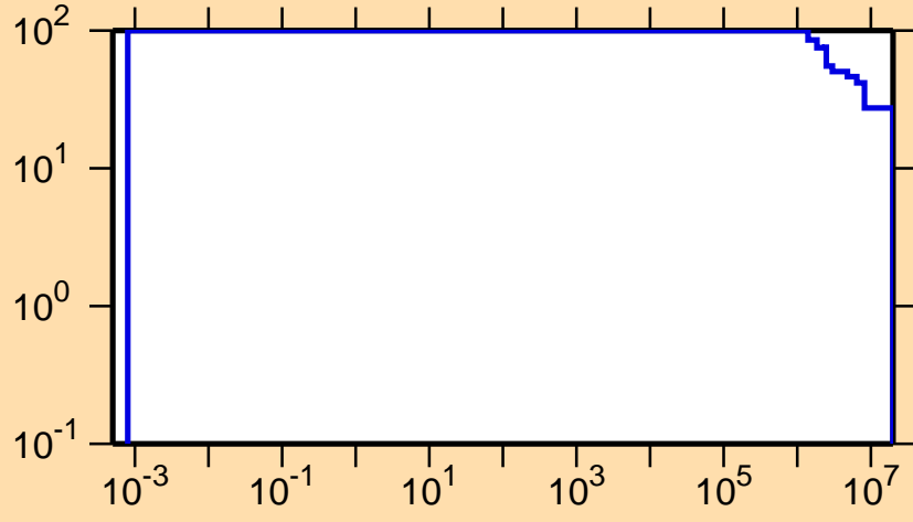
\Delta\sigma/\sigma vs. E for ^{188}\text{Au}(n,p)
