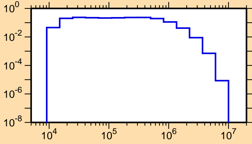
\sigma vs. E for ^{189}\text{Au}(n,n_1)
