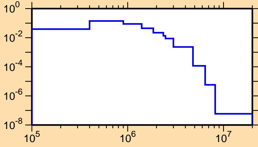
\sigma vs. E for ^{189}\text{Au}(n,n_2)
