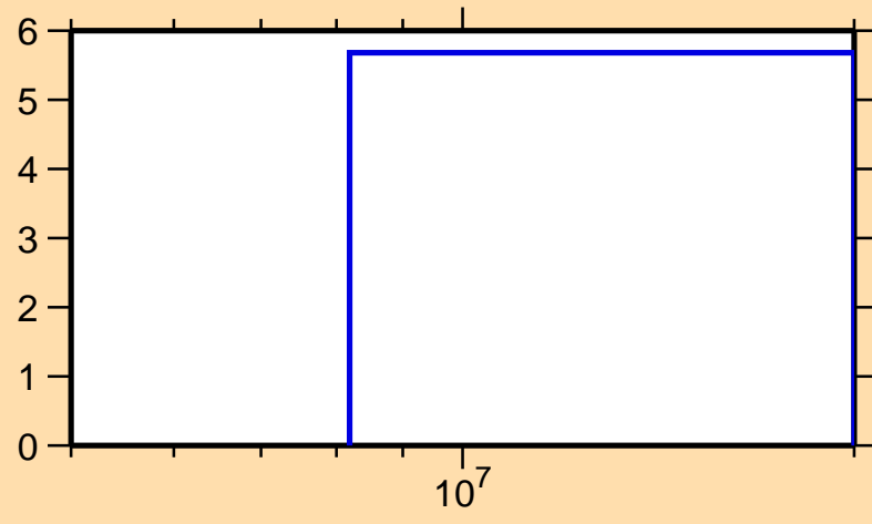
\Delta\sigma/\sigma vs. E for ^{189}\text{Au}(n,\text{el.})
