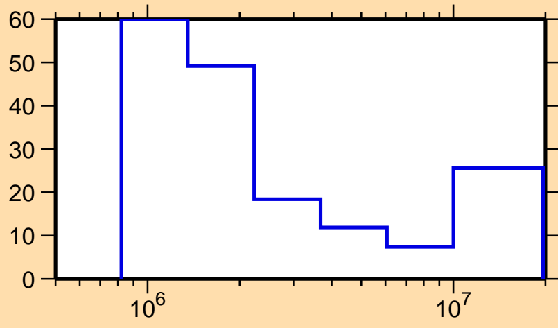
\Delta\sigma/\sigma vs. E for ^{189}\text{Au}(n,n\text{cont.})
