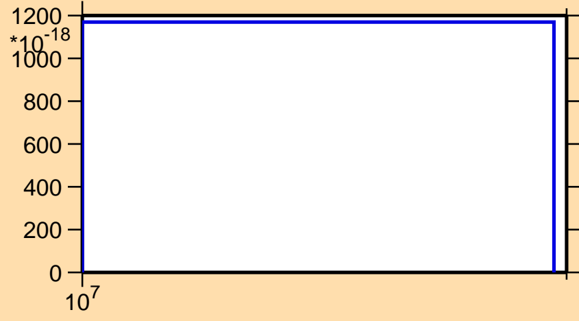
\sigma vs. E for ^{189}\text{Au}(n,pt)
