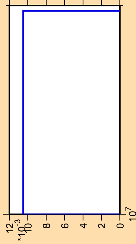
\Delta\sigma/\sigma vs. E for ^{189}\text{Au}(n,pt)
