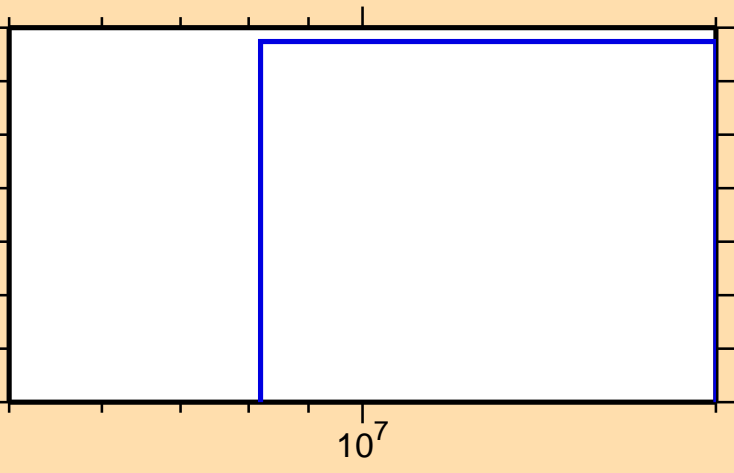
\sigma vs. E for ^{189}\text{Au}(n,\text{pt})
