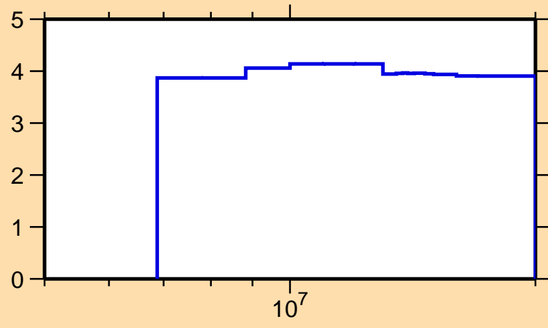
\Delta\sigma/\sigma vs. E for ^{190}\text{Au}(n,\text{nonel.})
