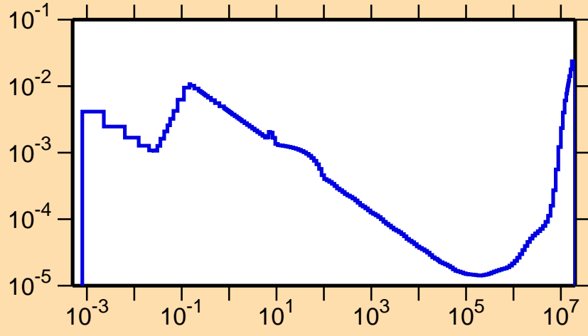
\sigma vs. E for ^{190}\text{Au}(n,\alpha)
