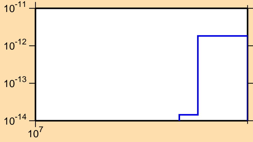
\sigma vs. E for ^{190}\text{Au}(n,pt)
