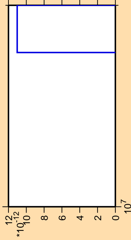
\Delta\sigma/\sigma vs. E for ^{190}\text{Au} (mt 42)
