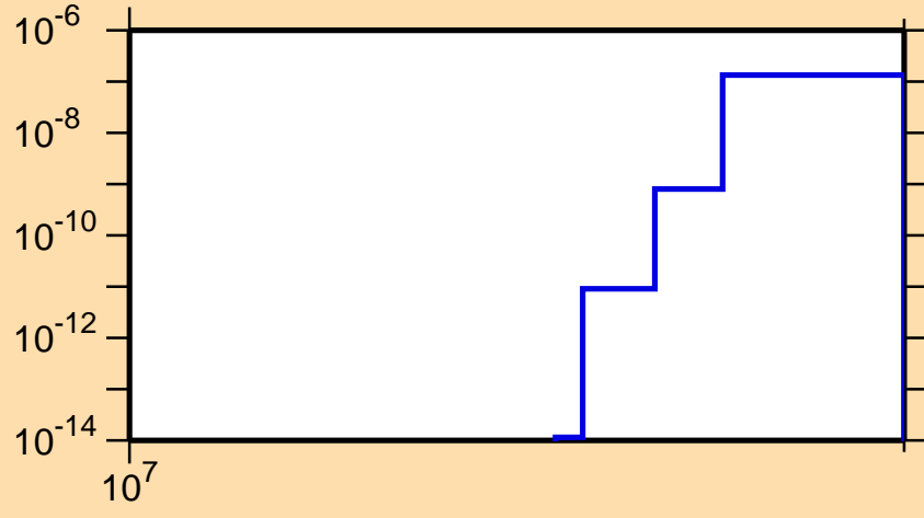
\sigma vs. E for ^{190}\text{Au}(n,nt)
