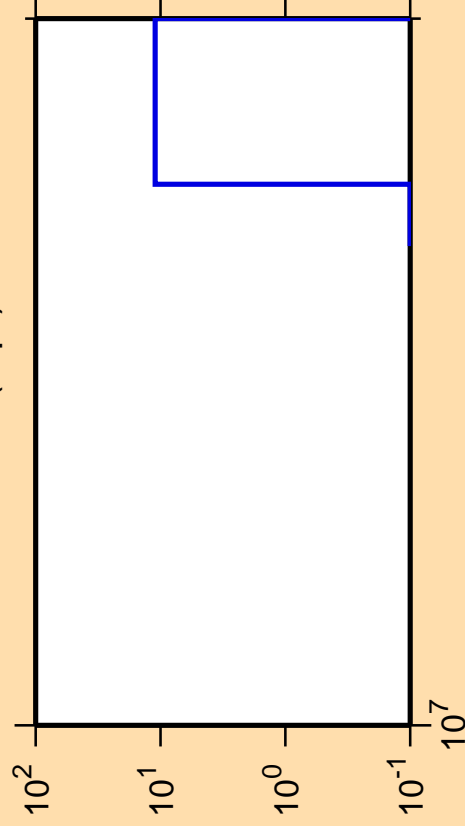
\Delta\sigma/\sigma vs. E for ^{190}\text{Au}(n,pt)
