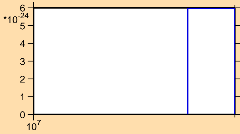
\sigma vs. E for ^{190}\text{Au} (mt 42)
