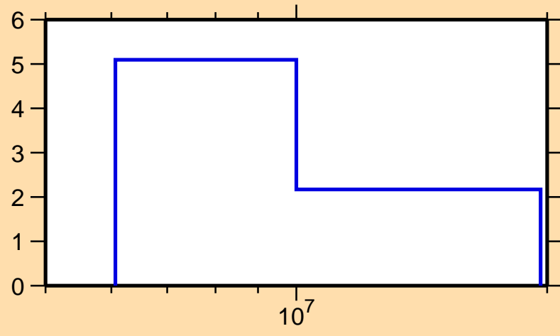
\Delta\sigma/\sigma vs. E for ^{190}\text{Au}(n,\text{tot.})
