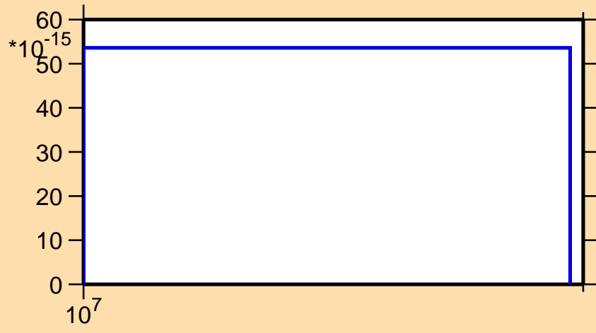
\sigma vs. E for ^{190}\text{Au} (mt 34)
