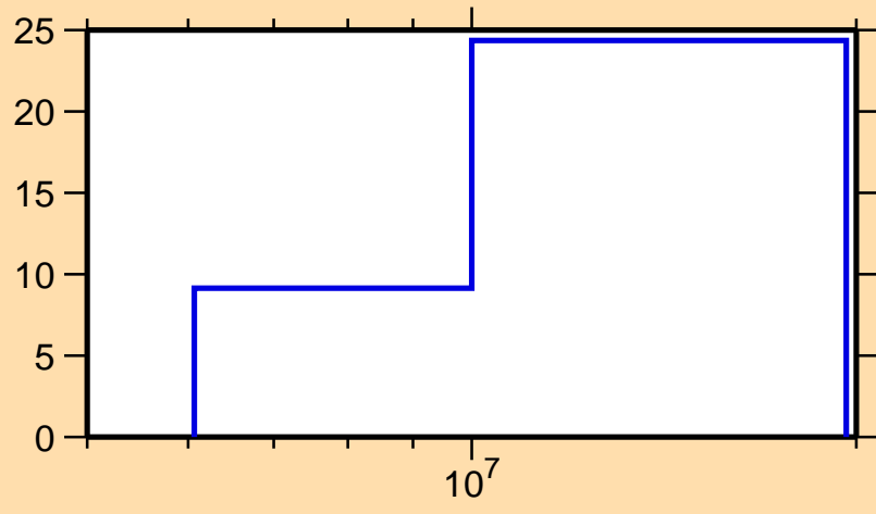
\Delta\sigma/\sigma vs. E for ^{190}\text{Au}(n,\text{inel.})
