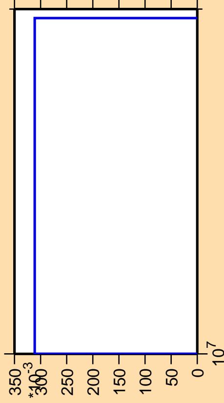
\Delta\sigma/\sigma vs. E for ^{190}\text{Au} (mt 34)
