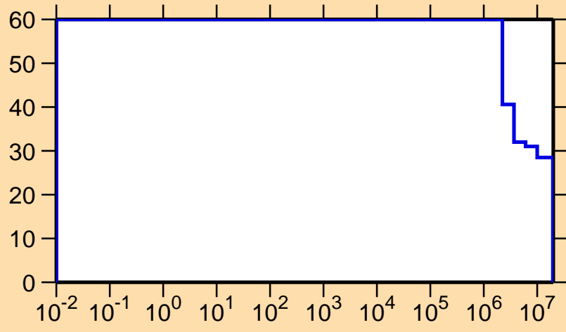
\Delta\sigma/\sigma vs. E for ^{190}\text{Au}(n,p)
