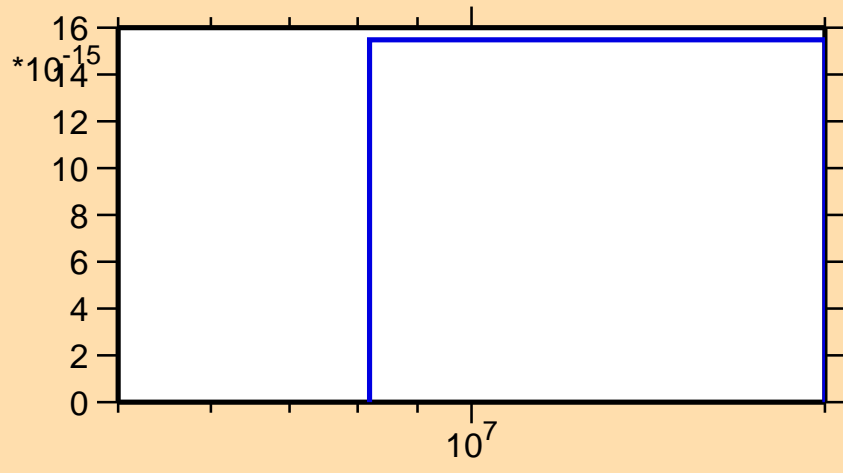
\sigma vs. E for ^{190}\text{Au}(n,\text{pt})
