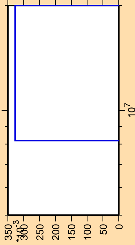
\Delta\sigma/\sigma vs. E for ^{190}\text{Au}(\text{mt } 34)
