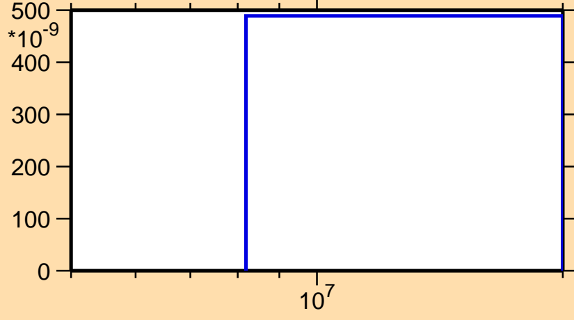
\sigma vs. E for ^{190}\text{Au}(n,nd)
