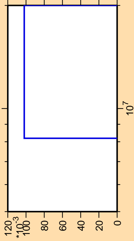
\Delta\sigma/\sigma vs. E for ^{190}\text{Au}(n,pd)
