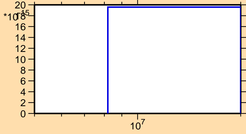
\sigma vs. E for ^{190}\text{Au}(n,pd)
