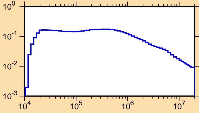
\sigma vs. E for ^{191}\text{Au}(n,n_1)
