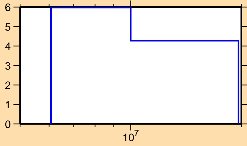
\Delta\sigma/\sigma vs. E for ^{191}\text{Au}(n,\text{el.})
