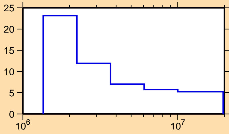
\Delta\sigma/\sigma vs. E for ^{191}\text{Au}(n,n\text{onel.})
