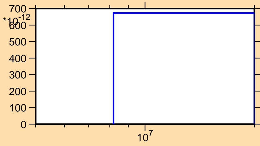
\sigma vs. E for ^{191}\text{Au}(n,nt)
