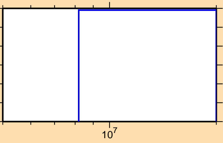
\sigma vs. E for ^{191}\text{Au}(n,\text{nd})
