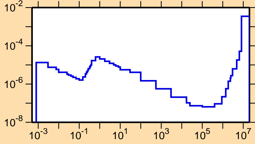
\sigma vs. E for ^{191}\text{Au}(n,\alpha)
