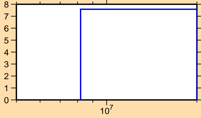
\Delta\sigma/\sigma vs. E for ^{191}\text{Au}(n,2n)
