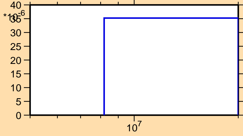
\sigma vs. E for ^{191}\text{Au}(n,t)
