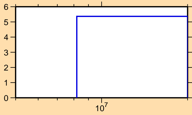
\Delta\sigma/\sigma vs. E for ^{191}\text{Au}(n,\text{nonel.})
