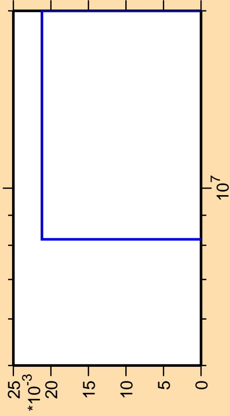
\Delta\sigma/\sigma vs. E for ^{191}\text{Au}(n,pd)
