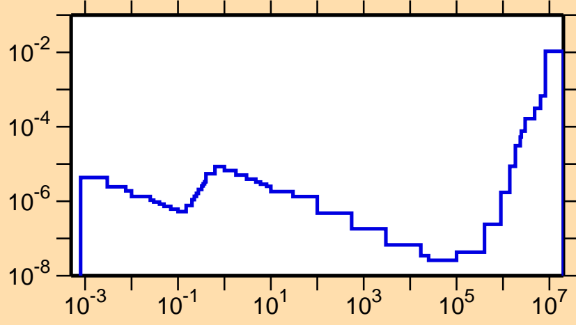
\sigma vs. E for ^{191}\text{Au}(n,p)
