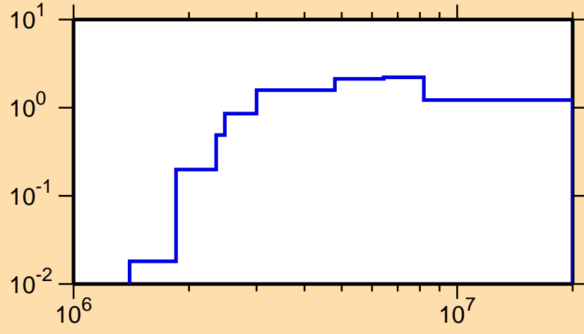
\sigma vs. E for ^{191}\text{Au}(n,n\text{cont.})
