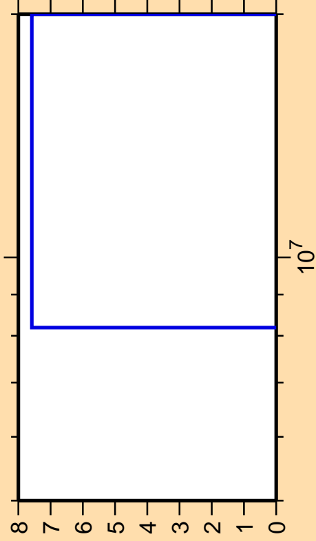
\Delta\sigma/\sigma vs. E for ^{191}\text{Au}(n,2n)
