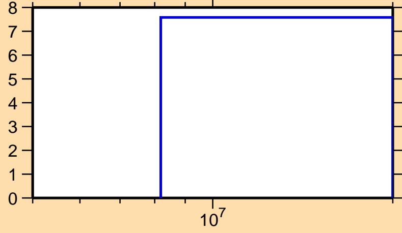
\Delta\sigma/\sigma vs. E for ^{191}\text{Au}(n,2n)
