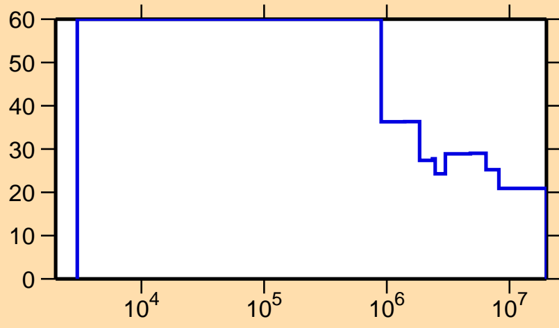
\Delta\sigma/\sigma vs. E for ^{191}\text{Au}(n,n_1)
