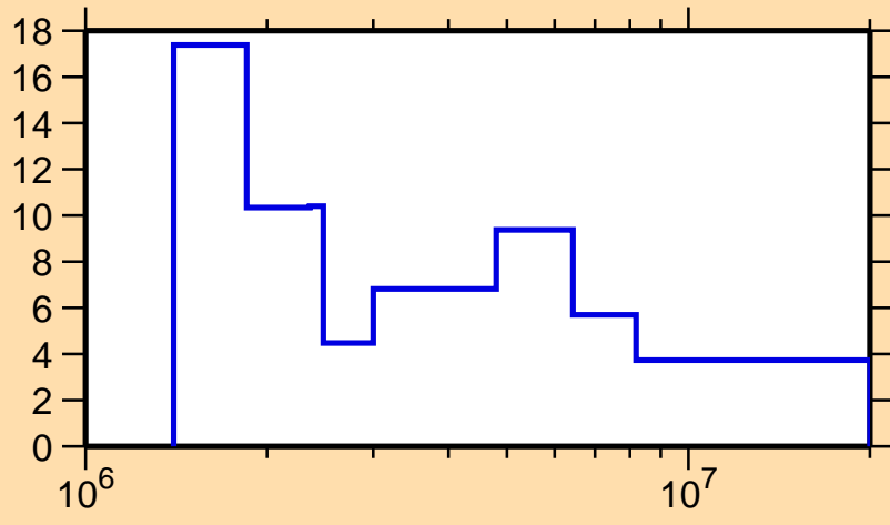
\Delta\sigma/\sigma vs. E for ^{191}\text{Au}(n, el.)
