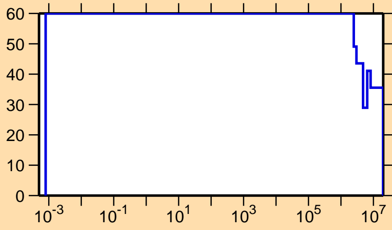
\Delta\sigma/\sigma vs. E for ^{191}\text{Au}(n,p)
