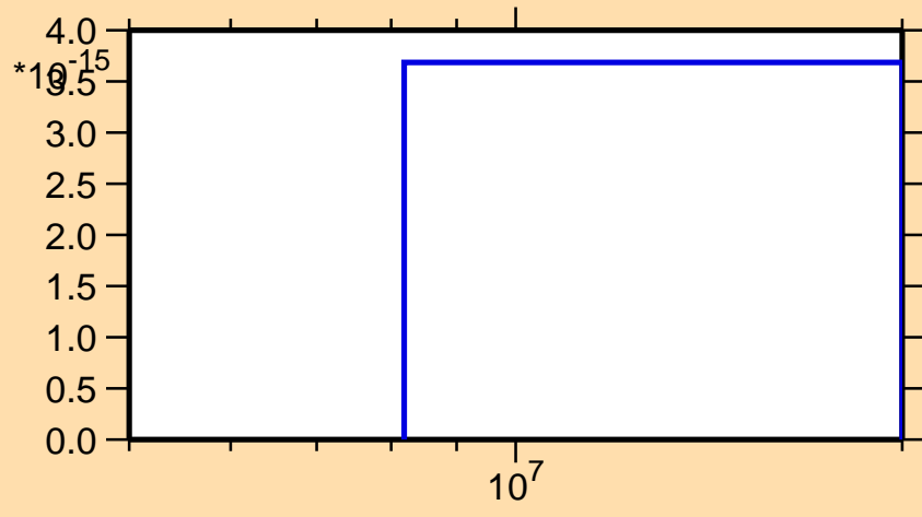
\sigma vs. E for ^{191}\text{Au}(n,pd)
