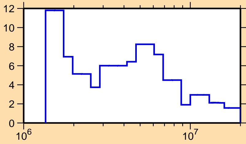
\Delta\sigma/\sigma vs. E for ^{193}\text{Au}(n, el.)
