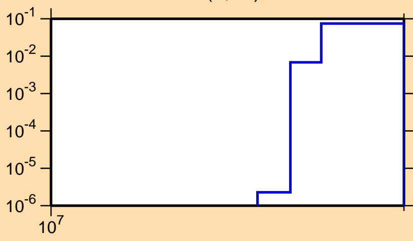
\sigma vs. E for ^{193}\text{Au}(n,3n)
