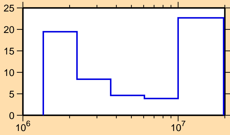
\Delta\sigma/\sigma vs. E for ^{193}\text{Au}(n,n\text{cont.})
