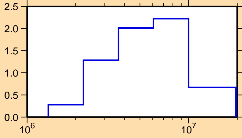
\sigma vs. E for ^{193}\text{Au}(n,n\text{cont.})
