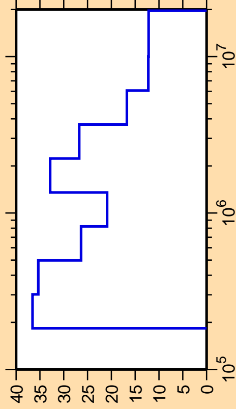
\Delta\sigma/\sigma vs. E for ^{193}\text{Au}(n,n_2)
