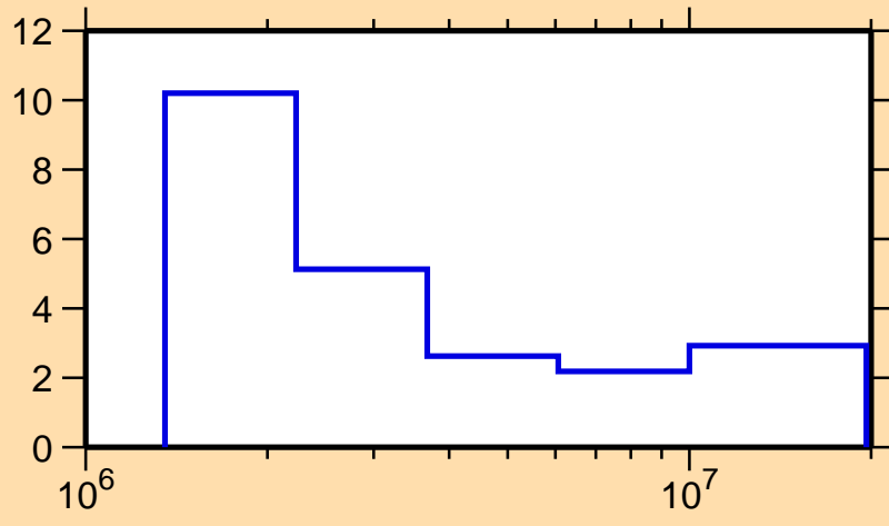
\Delta\sigma/\sigma vs. E for ^{193}\text{Au}(n,n\text{onel.})
