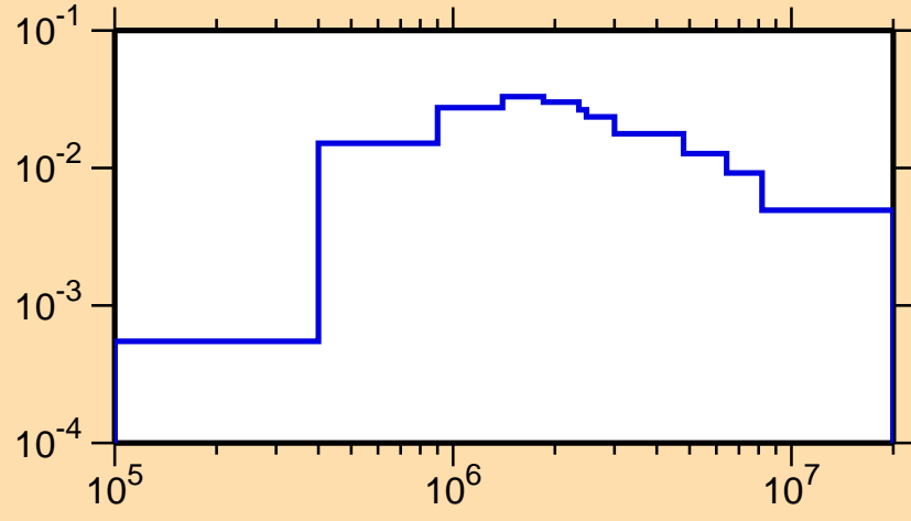
\sigma vs. E for ^{193}\text{Au}(n,n_4)
