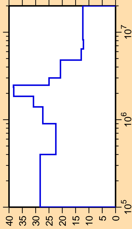
\Delta\sigma/\sigma vs. E for ^{193}\text{Au}(n,n_4)
