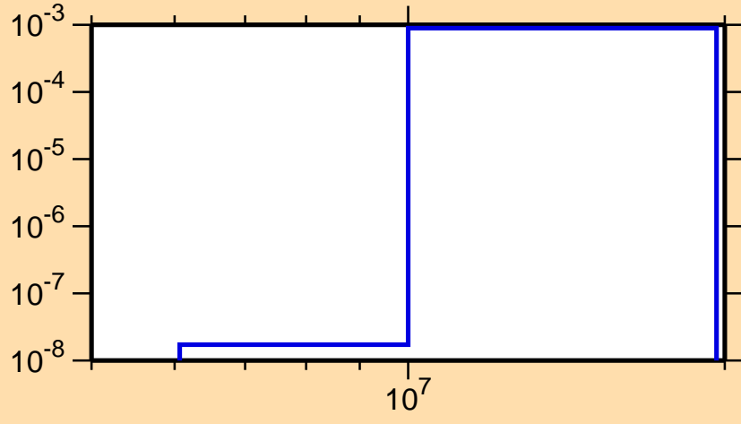
\sigma vs. E for ^{193}\text{Au}(n,d)
