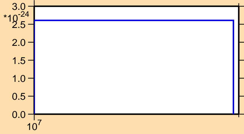
\sigma vs. E for ^{193}\text{Au} (mt 42)
