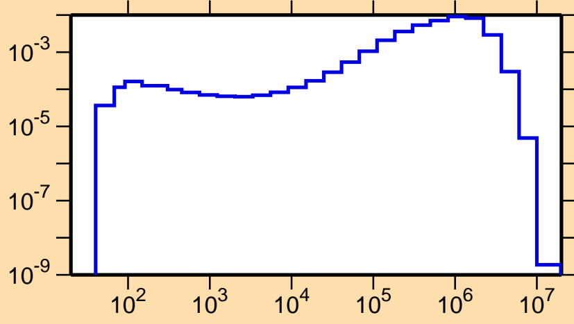
\sigma vs. E for ^{193}\text{Au}(n,n_3)
