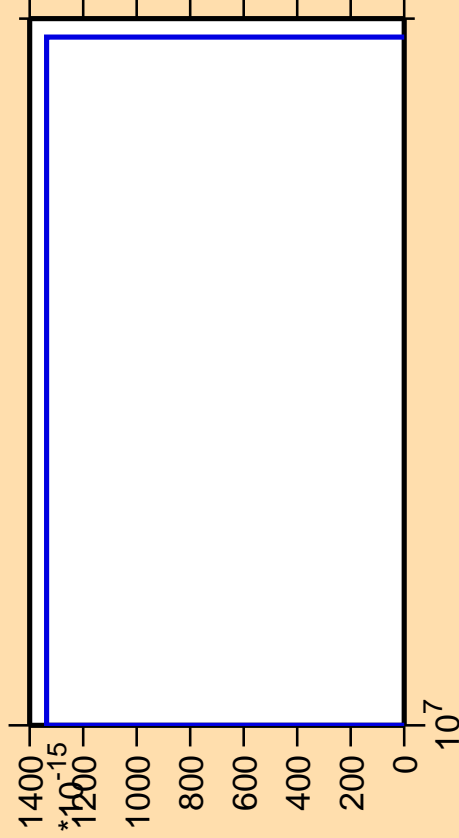
\Delta\sigma/\sigma vs. E for ^{193}\text{Au} (mt 42)
