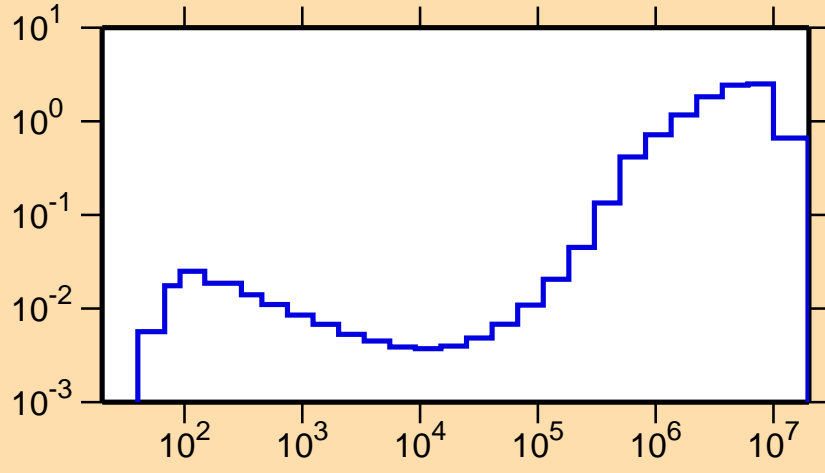
\sigma vs. E for ^{193}\text{Au}(n,\text{inel.})
