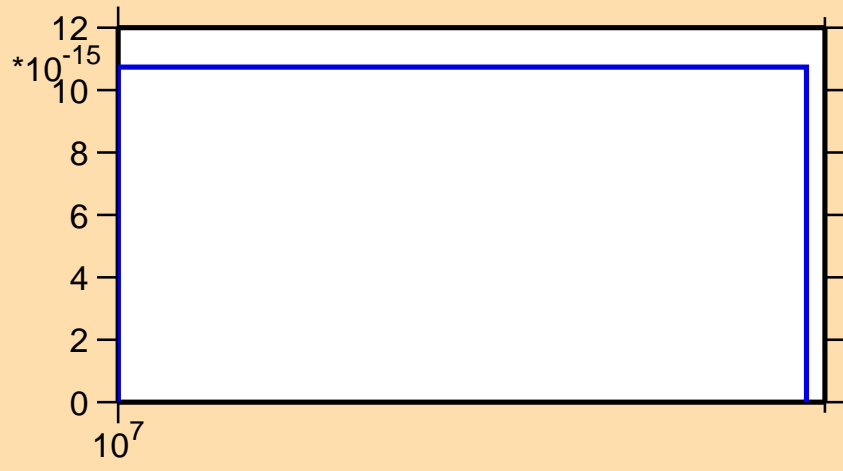
\sigma vs. E for ^{193}\text{Au} (mt 45)
