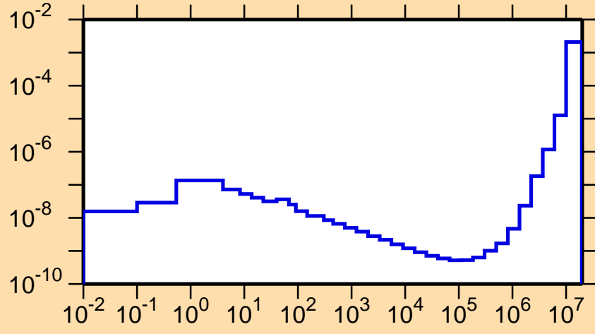
\sigma vs. E for ^{193}\text{Au}(n,\alpha)
