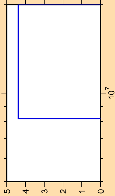
\Delta\sigma/\sigma vs. E for ^{193}\text{Au}(n,2n)
