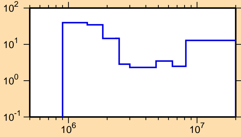
\Delta\sigma/\sigma vs. E for ^{193}\text{Au}(n,n\text{cont.})
