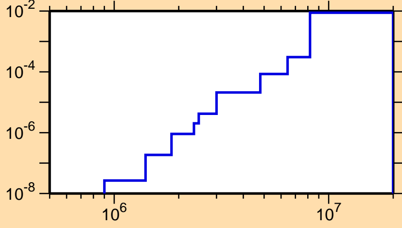
\sigma vs. E for ^{193}\text{Au}(n,p)
