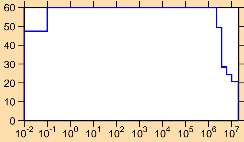
\Delta\sigma/\sigma vs. E for ^{194}\text{Au}(n,p)
