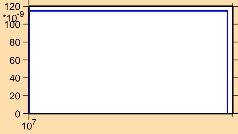
\sigma vs. E for ^{194}\text{Au}(n,\text{nd})
