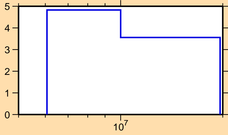
\Delta\sigma/\sigma vs. E for ^{194}\text{Au}(n,\text{el.})
