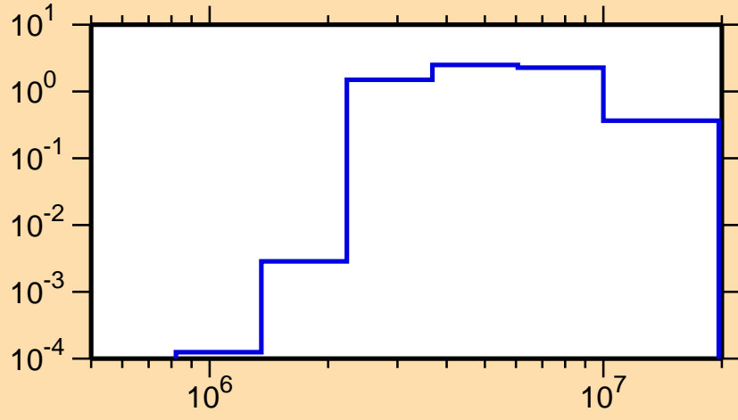
\sigma vs. E for ^{194}\text{Au}(n,n\text{cont.})
