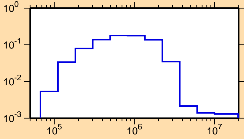
\sigma vs. E for ^{194}\text{Au}(n,n_2)
