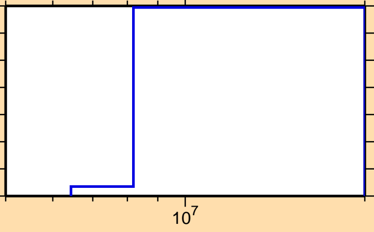
\sigma vs. E for ^{194}\text{Au}(n,np)
