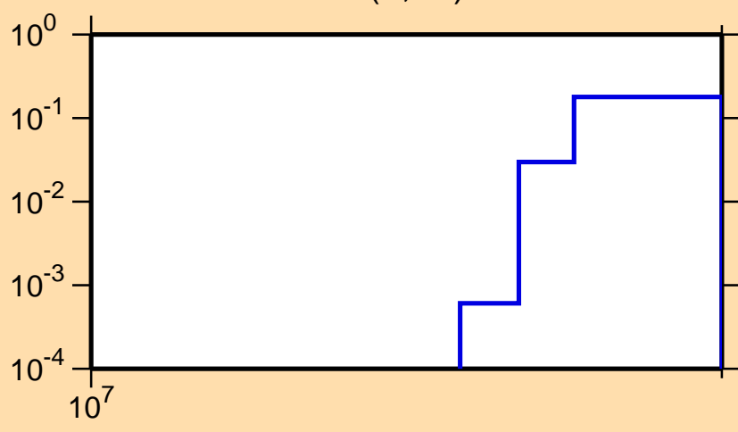
\sigma vs. E for ^{195}\text{Au}(n,3n)
