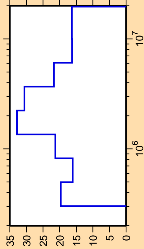
\Delta\sigma/\sigma vs. E for ^{195}\text{Au}(n,n_4)
