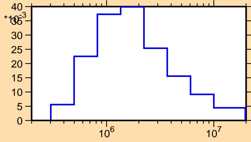
\sigma vs. E for ^{195}\text{Au}(n,n_4)
