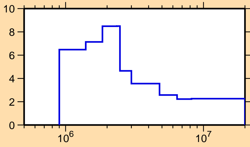
\Delta\sigma/\sigma vs. E for ^{195}\text{Au}(n,n\text{onel.})
