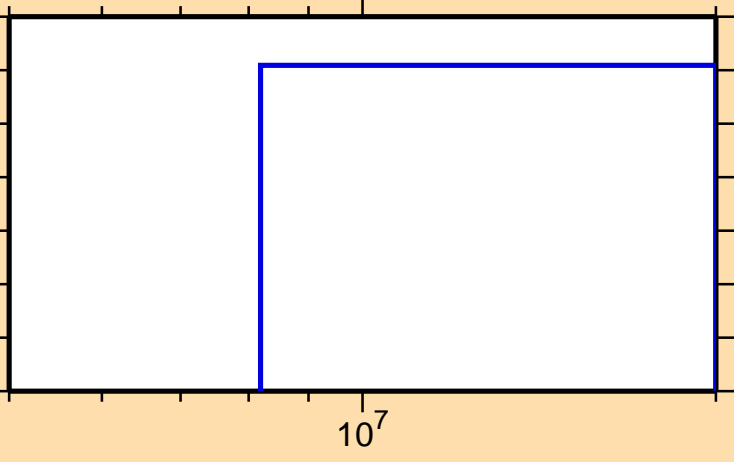
\sigma vs. E for ^{195}\text{Au}(n,\text{nd})
