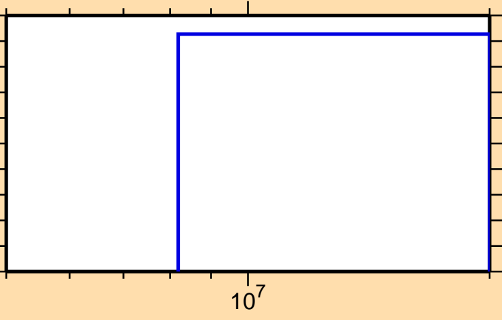
\sigma vs. E for ^{195}\text{Au}(n,t)
