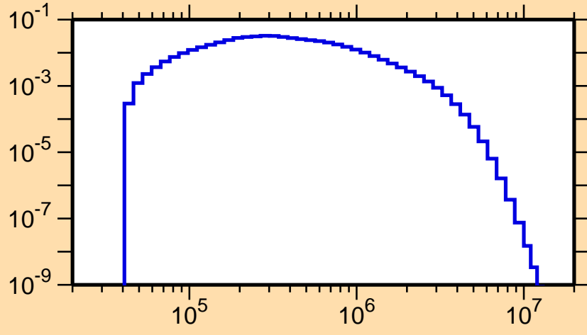
\sigma vs. E for ^{196}\text{Au}(n,n_2)
