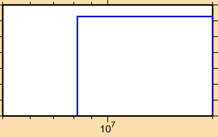
\sigma vs. E for ^{196}\text{Au}(n,nt)
