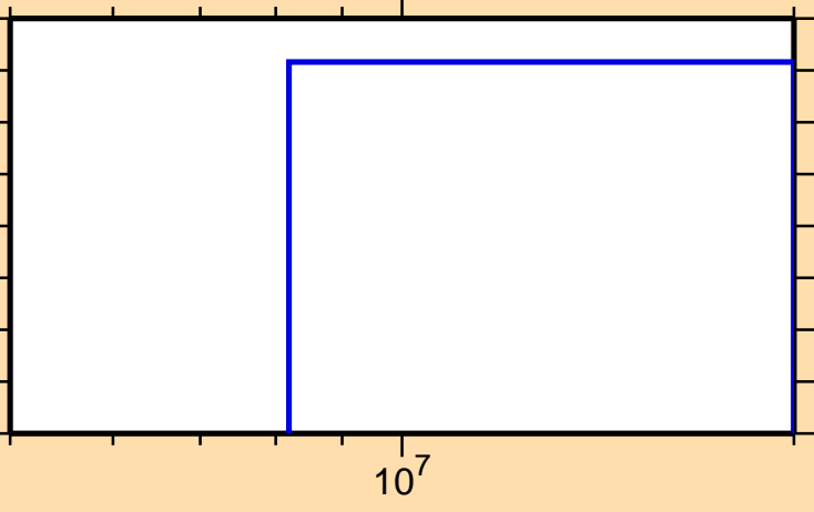
\sigma vs. E for ^{196}\text{Au}(n,2np)
