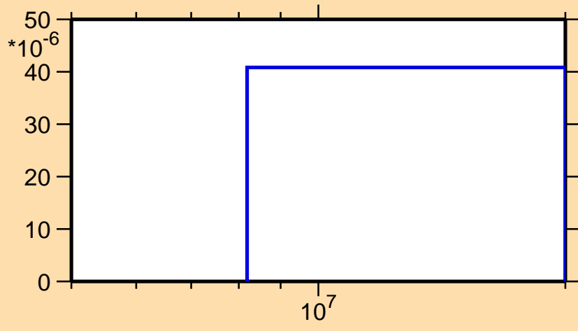
\sigma vs. E for ^{196}\text{Au}(n,t)
