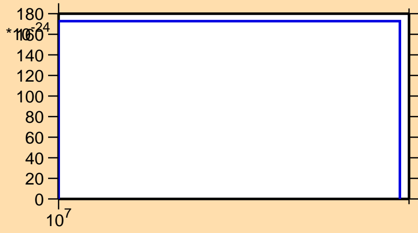
\sigma vs. E for ^{196}\text{Au} (mt 42)
