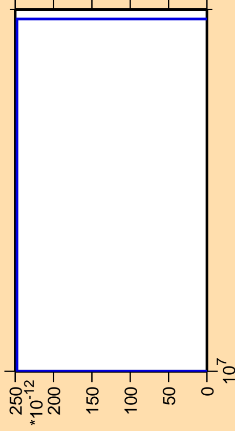
\Delta\sigma/\sigma vs. E for ^{196}\text{Au} (mt 42)
