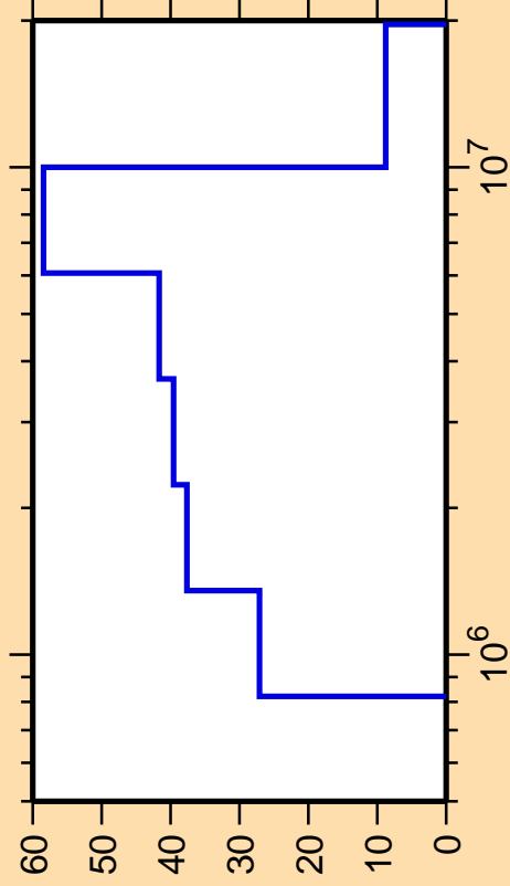
\Delta\sigma/\sigma vs. E for ^{196}\text{Au}(n,n_2)
