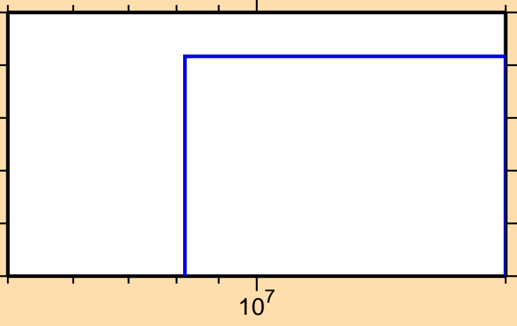
\sigma vs. E for ^{196}\text{Au}(n,3n)
