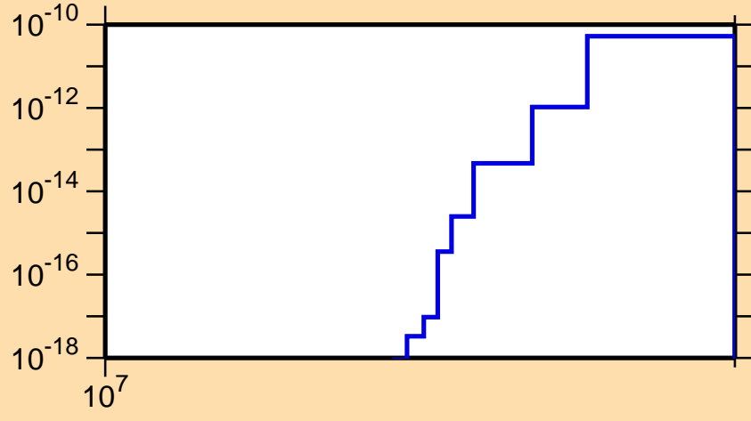
\sigma vs. E for ^{197}\text{Au}(n,\text{He}3)
