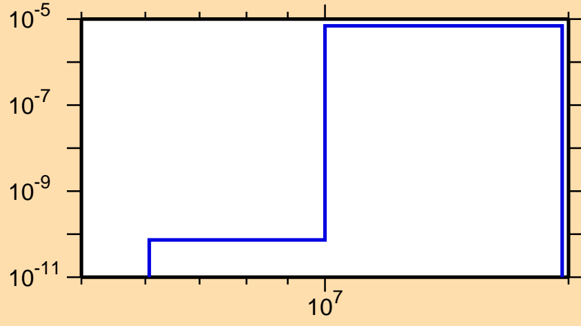
\sigma vs. E for ^{197}\text{Au}(n,n\alpha)
