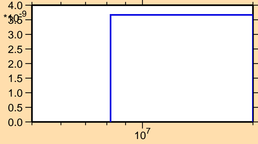
\sigma vs. E for ^{197}\text{Au}(n,nd)
