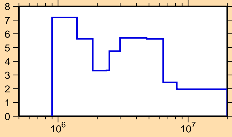
\Delta\sigma/\sigma vs. E for ^{197}\text{Au}(n, el.)
