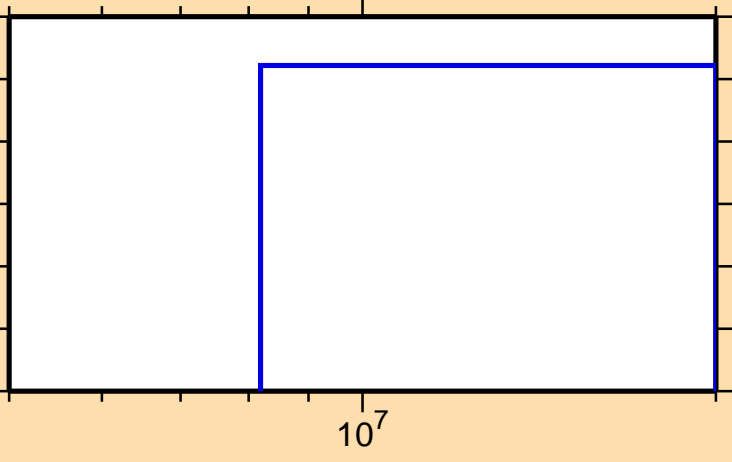
\sigma vs. E for ^{197}\text{Au}(n,2np)
