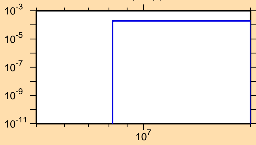
\sigma vs. E for ^{197}\text{Au}(n,np)
