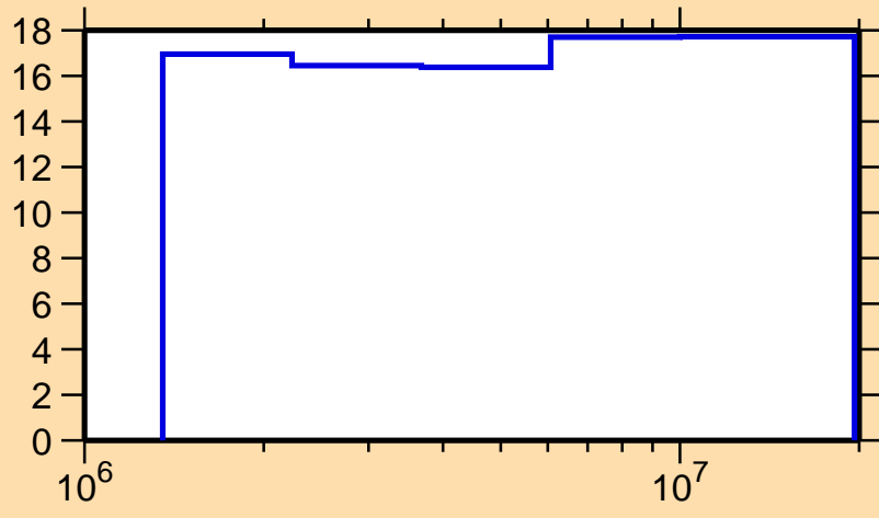
\Delta\sigma/\sigma vs. E for ^{198}\text{Au}(n,n_1)
