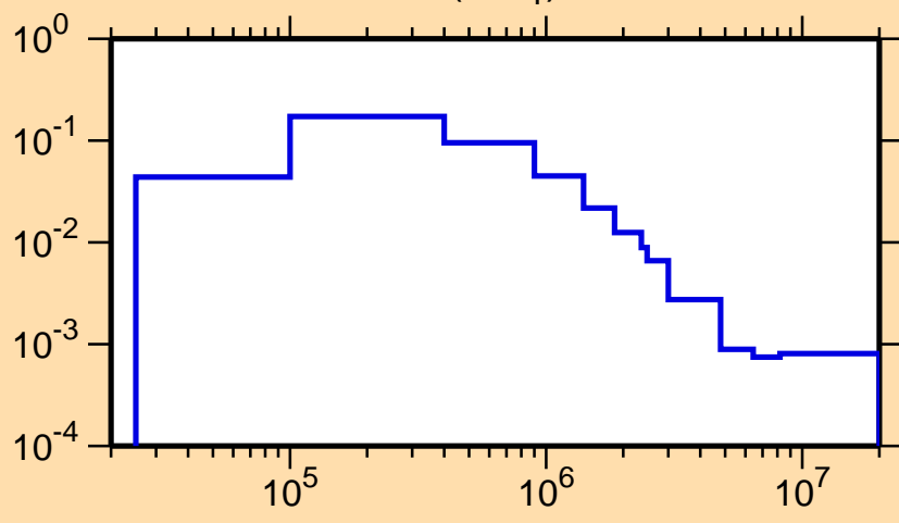
\sigma vs. E for ^{198}\text{Au}(n,n_1)
