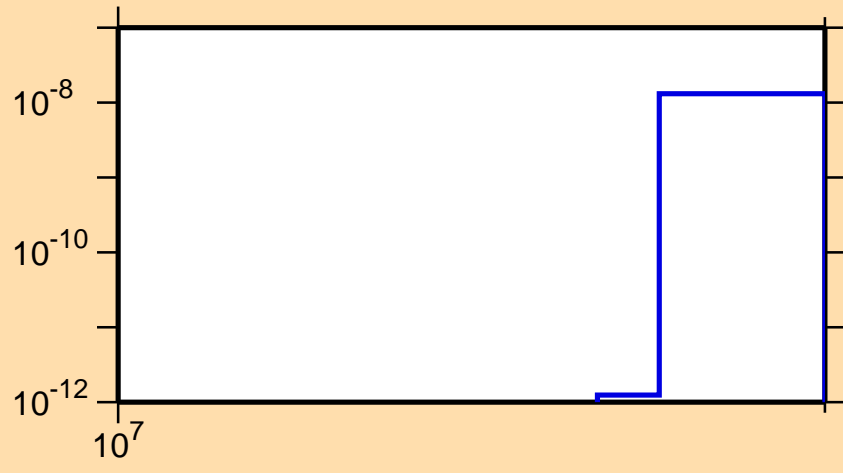
\sigma vs. E for ^{199}\text{Au}(n,2np)
