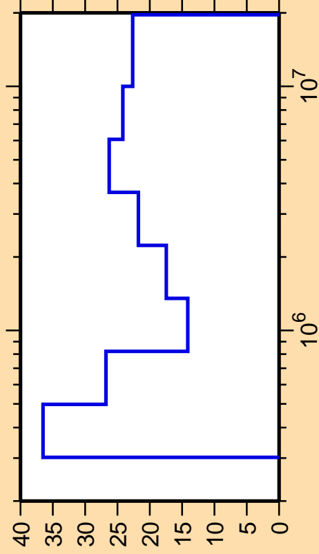
\Delta\sigma/\sigma vs. E for ^{199}\text{Au}(n,n_2)
