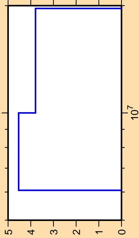
\Delta\sigma/\sigma vs. E for ^{199}\text{Au}(n,2n)
