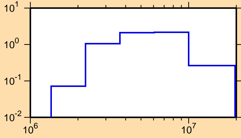
\sigma vs. E for ^{199}\text{Au}(n,n\text{cont.})
