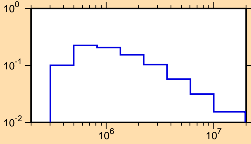
\sigma vs. E for ^{199}\text{Au}(n,n_3)
