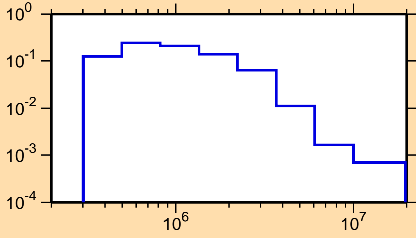
\sigma vs. E for ^{199}\text{Au}(n,n_2)
