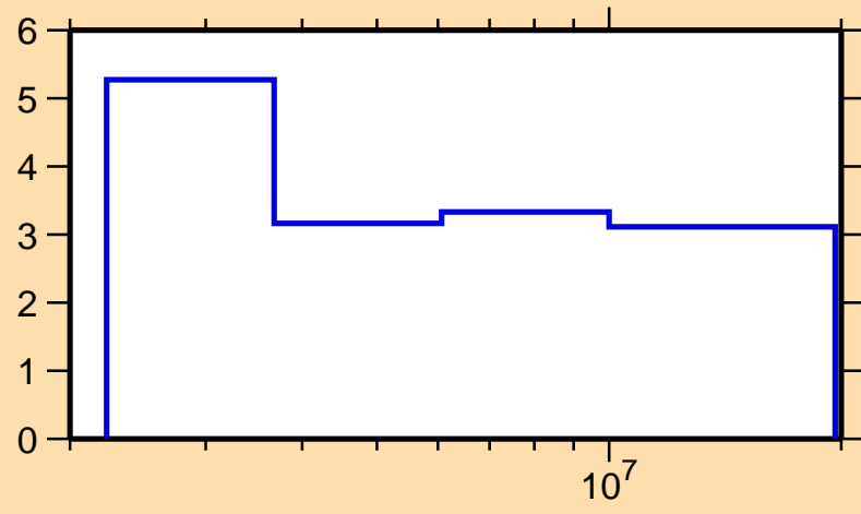
\Delta\sigma/\sigma vs. E for ^{199}\text{Au}(n,\text{nonel.})
