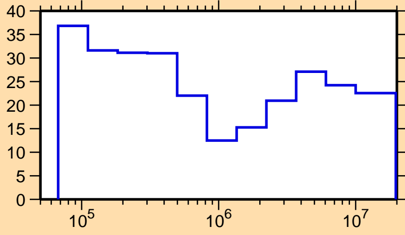
\Delta\sigma/\sigma vs. E for ^{199}\text{Au}(n,n_1)
