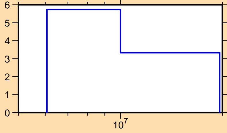
\Delta\sigma/\sigma vs. E for ^{199}\text{Au}(n,\text{el.})
