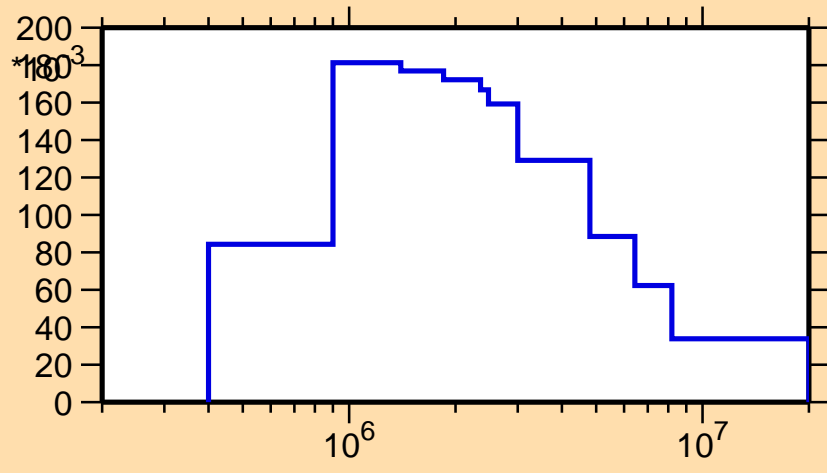
\sigma vs. E for ^{199}\text{Au}(n,n_4)
