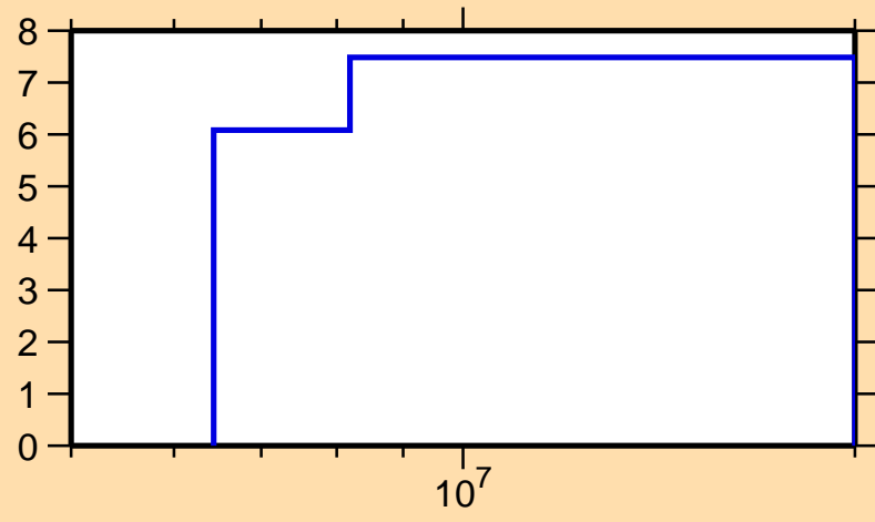
\Delta\sigma/\sigma vs. E for ^{199}\text{Au}(n,\text{inel.})
