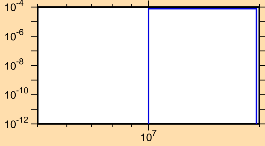
\sigma vs. E for ^{200}\text{Au}(n,np)
