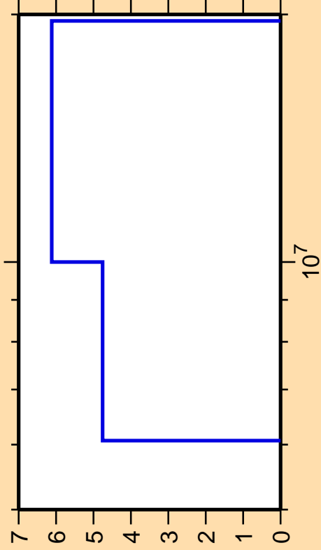
\Delta\sigma/\sigma vs. E for ^{200}\text{Au}(n,2n)
