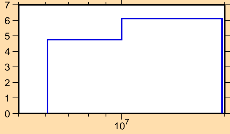
\Delta\sigma/\sigma vs. E for ^{200}\text{Au}(n,2n)
