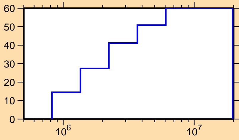
\Delta\sigma/\sigma vs. E for ^{200}\text{Au}(n,n_1)
