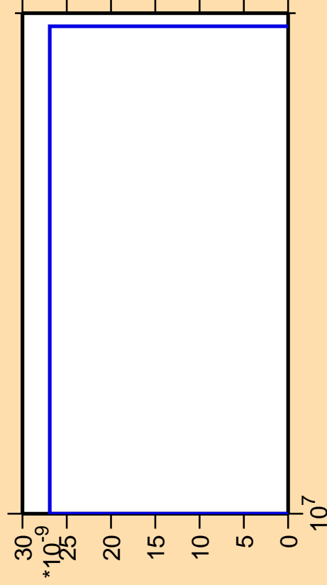
\Delta\sigma/\sigma vs. E for ^{200}\text{Au} (mt 11)
