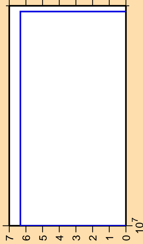
\Delta\sigma/\sigma vs. E for ^{200}\text{Au}(n,3n)
