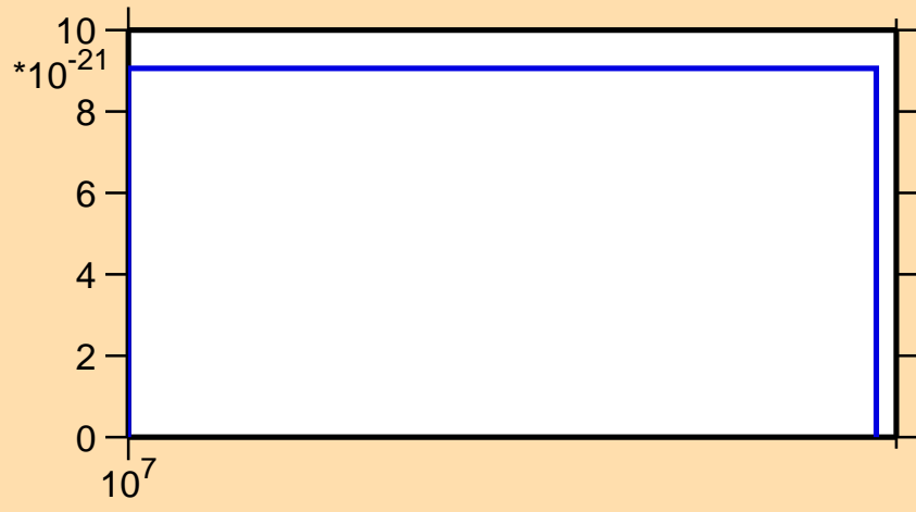
\sigma vs. E for ^{200}\text{Au} (mt 11)
