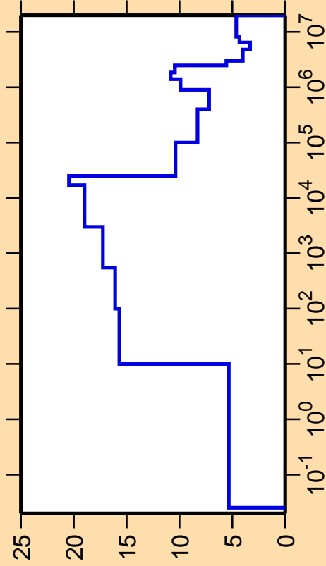
\Delta\sigma/\sigma vs. E for ^{200}\text{Au}(n,\text{nonel.})
