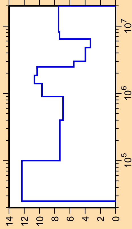
\Delta\sigma/\sigma vs. E for ^{200}\text{Au}(n,\text{inel.})
