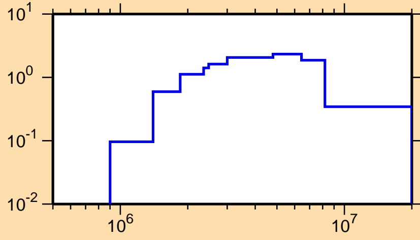
\sigma vs. E for ^{200}\text{Au}(n,n\text{cont.})
