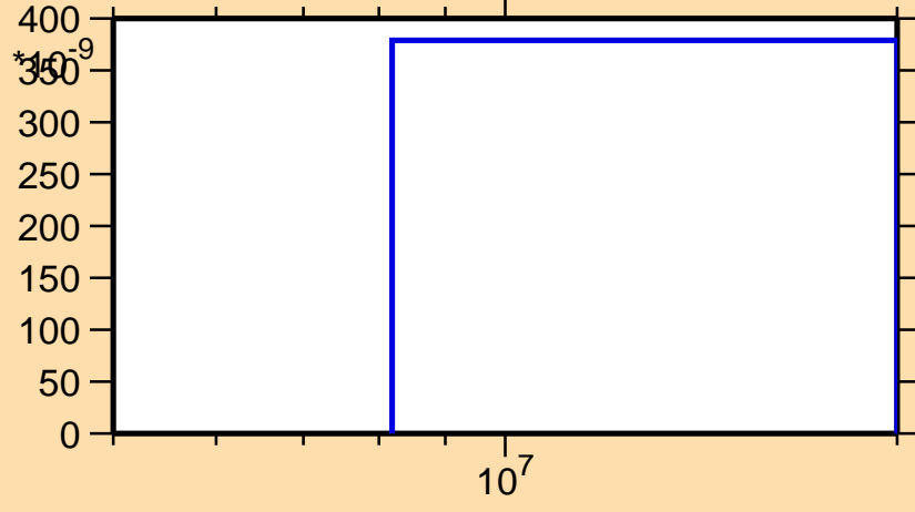
\sigma vs. E for ^{200}\text{Au}(n,n\alpha)
