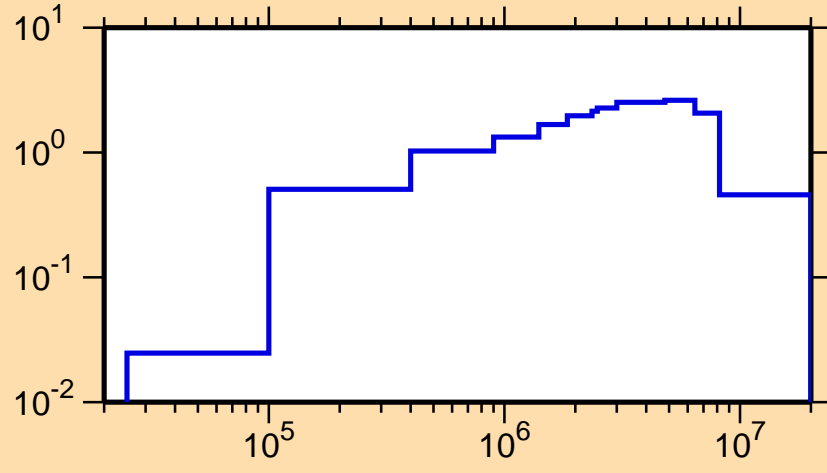
\sigma vs. E for ^{200}\text{Au}(n,\text{inel.})
