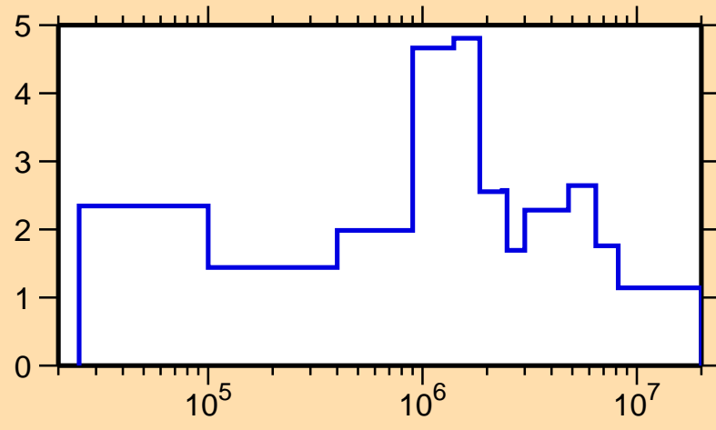
\Delta\sigma/\sigma vs. E for ^{200}\text{Au}(n,\text{el.})
