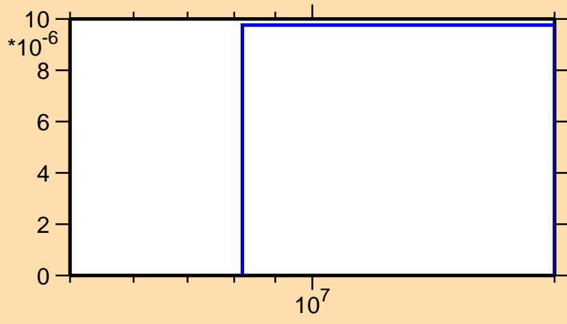
\sigma vs. E for ^{200}\text{Au}(n,t)
