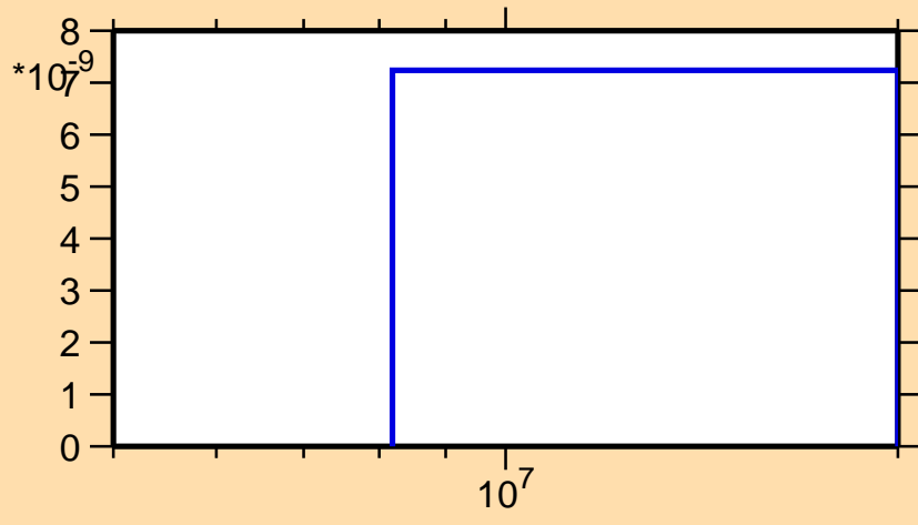
\sigma vs. E for ^{200}\text{Au}(n,nd)
