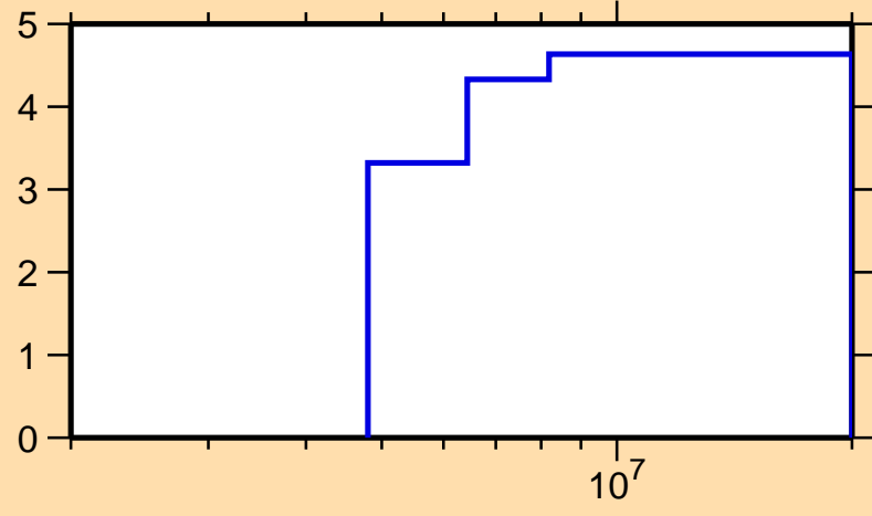
\Delta\sigma/\sigma vs. E for ^{200}\text{Au}(n,\text{nonel.})
