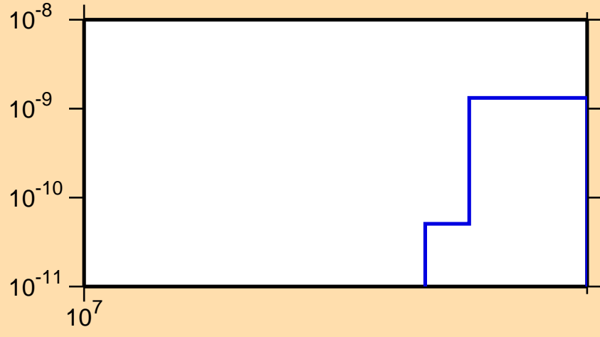
\sigma vs. E for ^{200}\text{Au}(n,2n\alpha)
