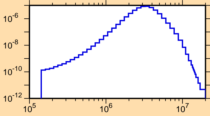
\sigma vs. E for ^{200}\text{Au}(n,n_4)
