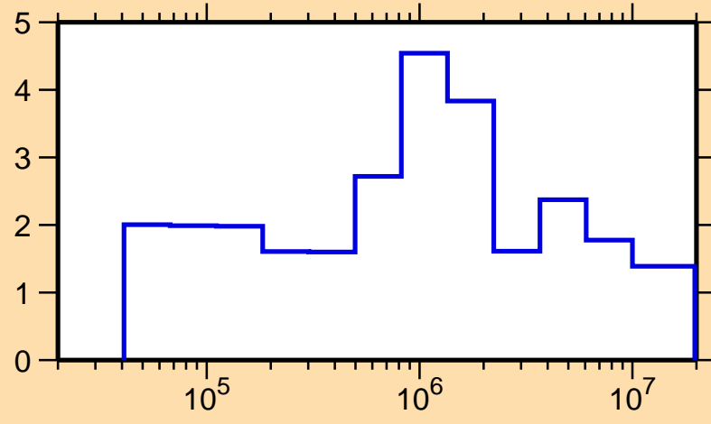
\Delta\sigma/\sigma vs. E for ^{200}\text{Au}(n, el.)
