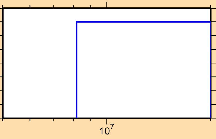
\sigma vs. E for ^{200}\text{Au}(n,\text{He}3)
