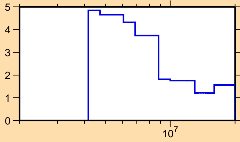
\Delta\sigma/\sigma vs. E for ^{201}\text{Au}(n,\text{tot.})
