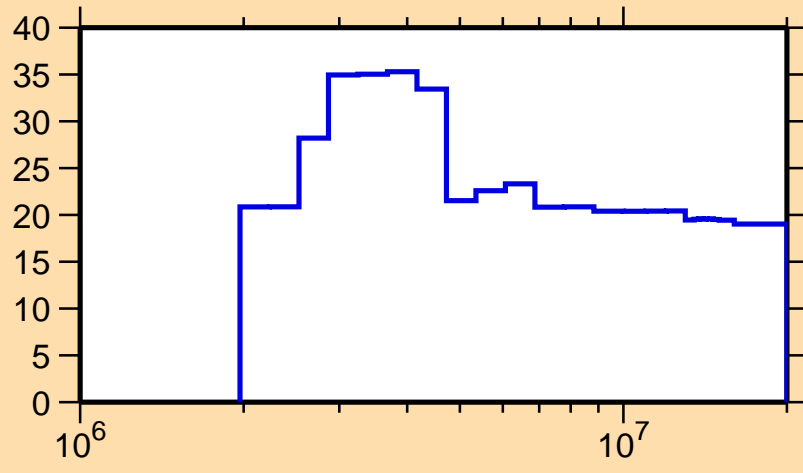
\Delta\sigma/\sigma vs. E for ^{201}\text{Au}(n,n_1)
