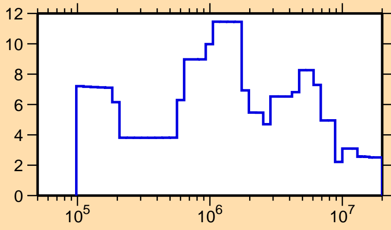
\Delta\sigma/\sigma vs. E for ^{201}\text{Au}(n,\text{el.})
