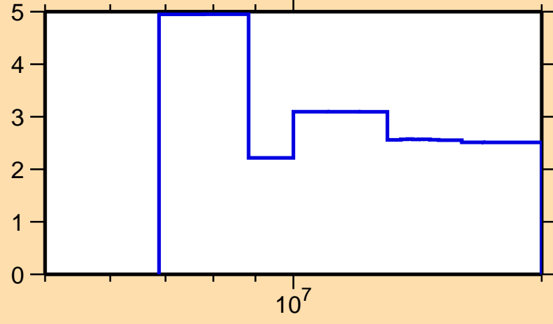
\Delta\sigma/\sigma vs. E for ^{201}\text{Au}(n,\text{el.})
