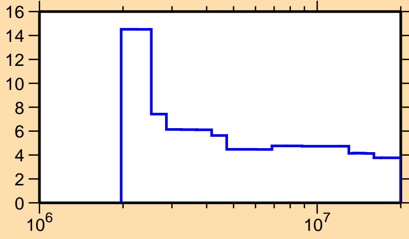
\Delta\sigma/\sigma vs. E for ^{201}\text{Au}(n,\text{nonel.})
