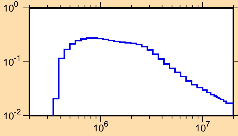
\sigma vs. E for ^{201}\text{Au}(n,n_2)
