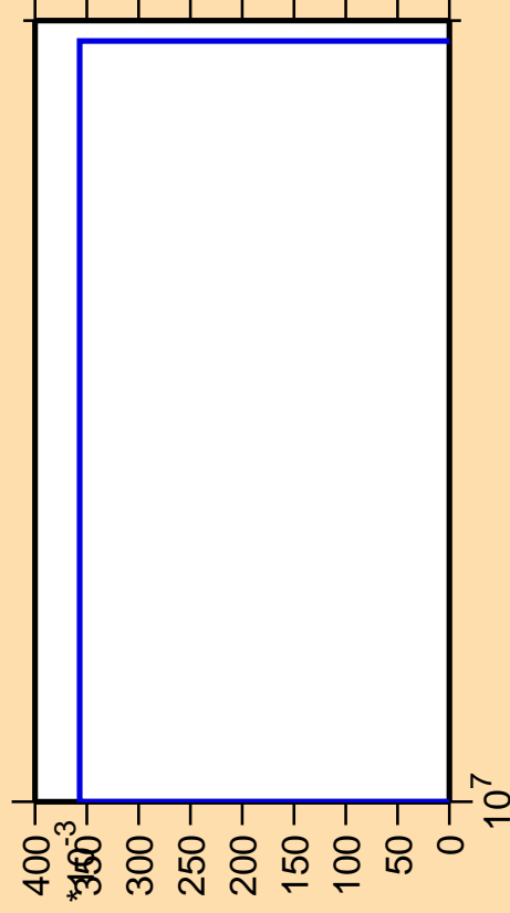
\Delta\sigma/\sigma vs. E for ^{201}\text{Au}(n,2n\alpha)
