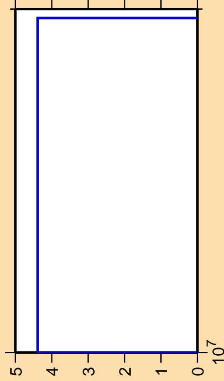
\Delta\sigma/\sigma vs. E for ^{201}\text{Au}(n,2np)
