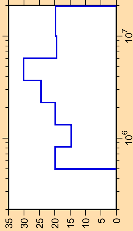
\Delta\sigma/\sigma vs. E for ^{201}\text{Au}(n,n_3)
