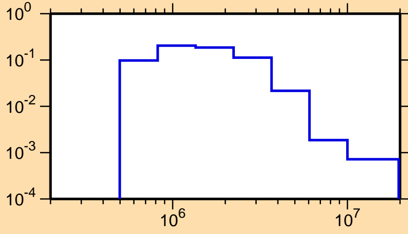
\sigma vs. E for ^{201}\text{Au}(n,n_3)
