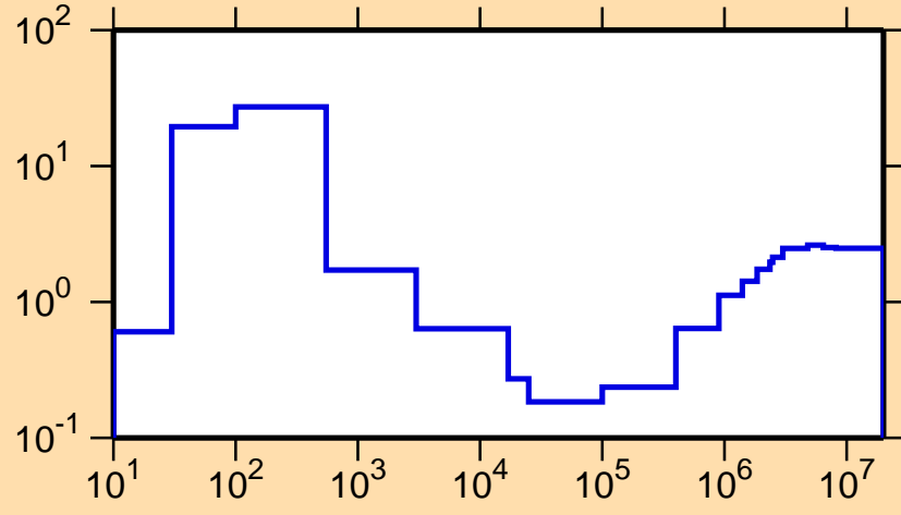
\sigma vs. E for ^{201}\text{Au}(n,\text{nonel.})
