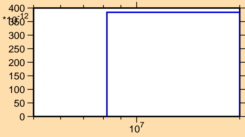
\sigma vs. E for ^{201}\text{Au}(n,nd)
