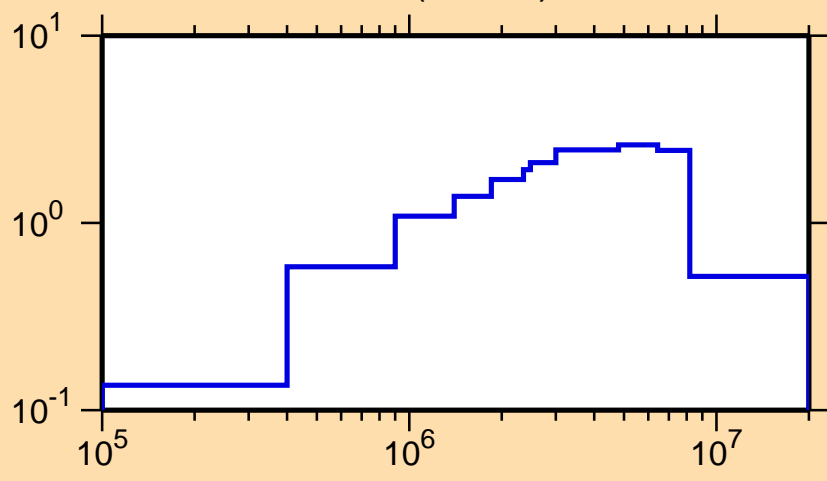
\sigma vs. E for ^{201}\text{Au}(n,\text{inel.})
