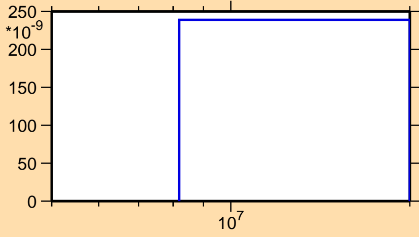
\sigma vs. E for ^{201}\text{Au}(n,n\alpha)
