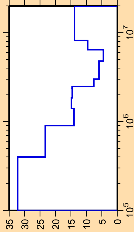
\Delta\sigma/\sigma vs. E for ^{201}\text{Au}(n,\text{inel.})
