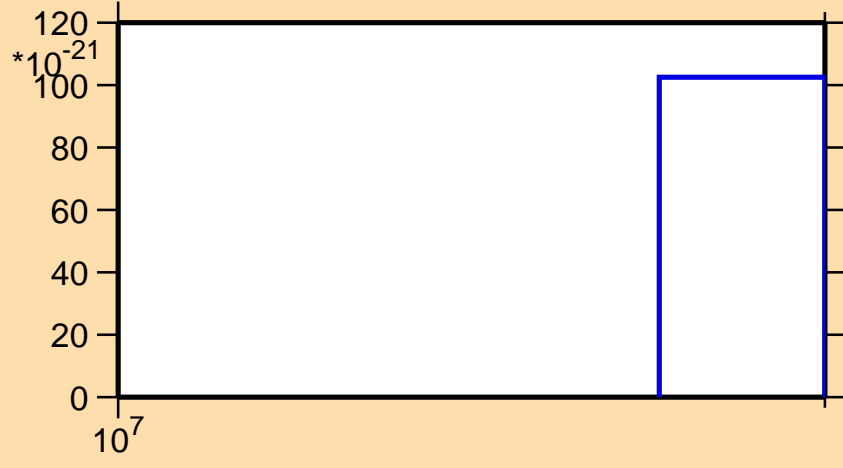
\sigma vs. E for ^{202}\text{Au} (mt 11)
