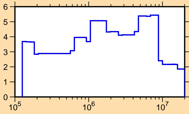
\Delta\sigma/\sigma vs. E for ^{202}\text{Au}(n,\text{tot.})
