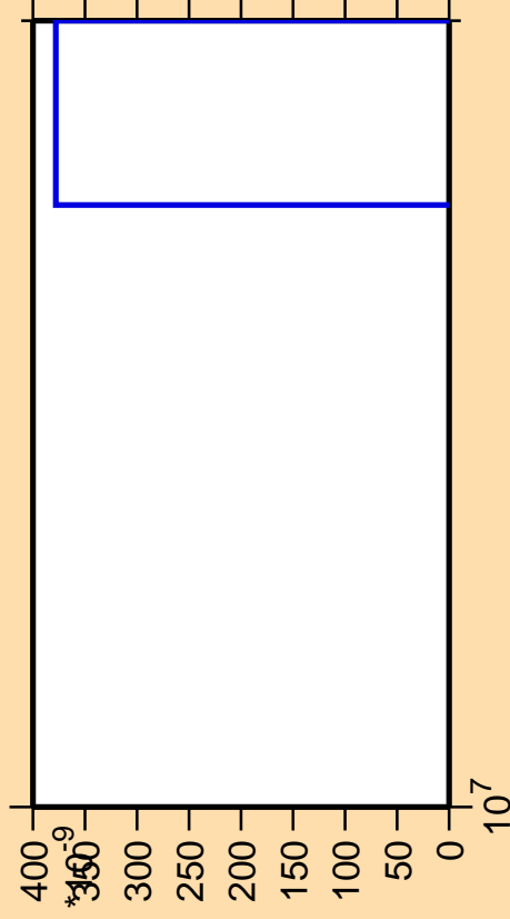
\Delta\sigma/\sigma vs. E for ^{202}\text{Au} (mt 11)
