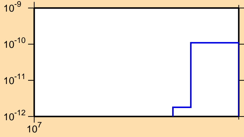
\sigma vs. E for ^{202}\text{Au}(n,2n\alpha)
