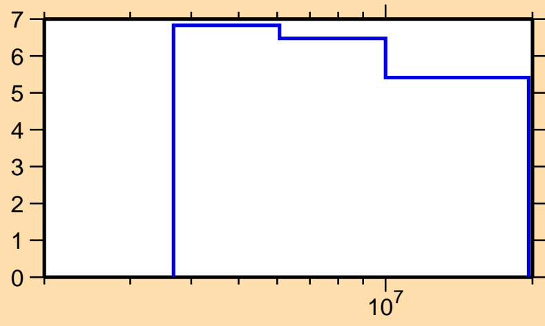
\Delta\sigma/\sigma vs. E for ^{202}\text{Au}(n,\text{el.})
