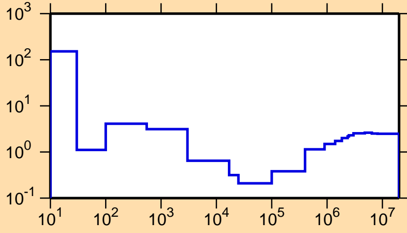
\sigma vs. E for ^{202}\text{Au}(n,\text{nonel.})
