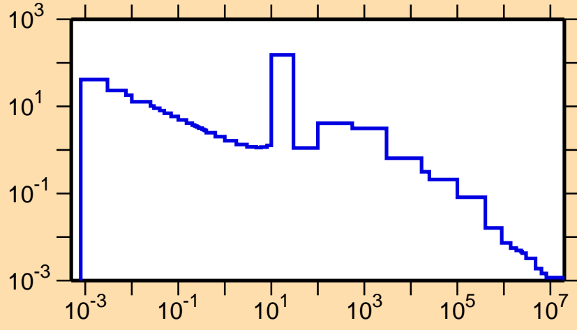
\sigma vs. E for ^{202}\text{Au}(n,\gamma)
