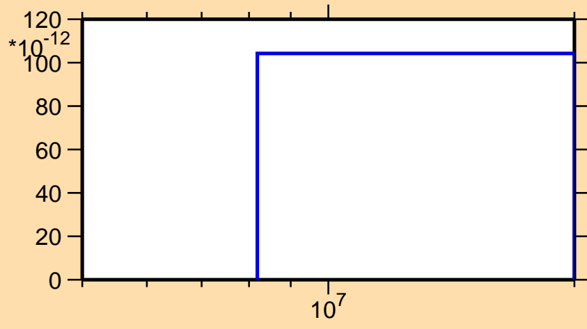
\sigma vs. E for ^{202}\text{Au}(n,2np)
