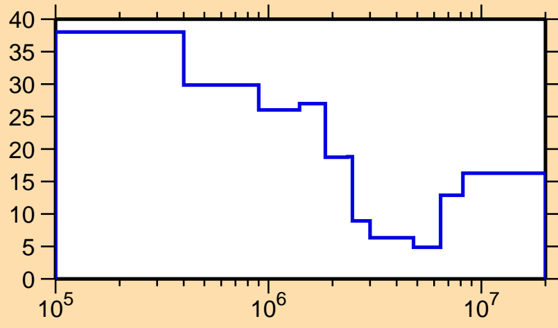
\Delta\sigma/\sigma vs. E for ^{202}\text{Au}(n,n\text{cont.})
