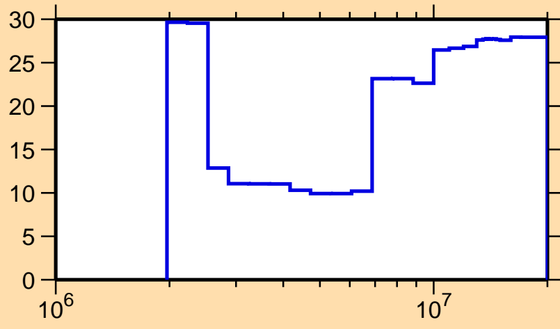
\Delta\sigma/\sigma vs. E for ^{203}\text{Au}(n,n\text{cont.})
