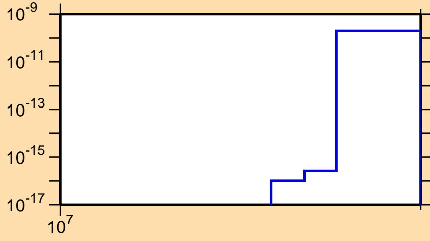
\sigma vs. E for ^{203}\text{Au}(n,2np)
