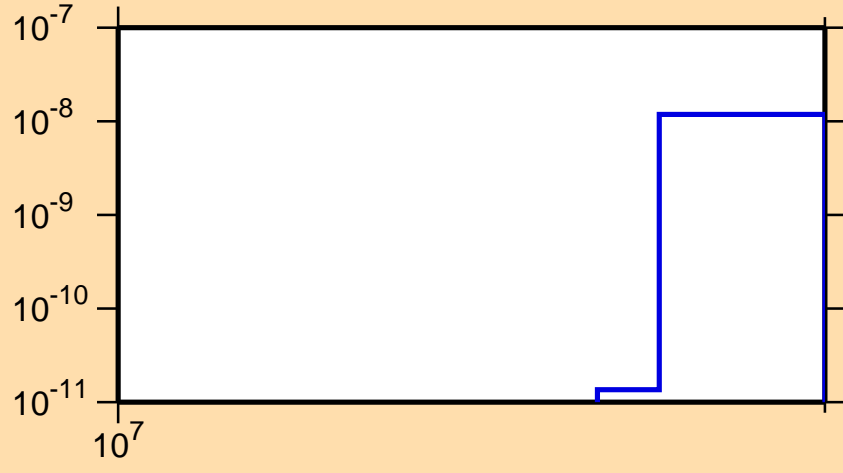
\sigma vs. E for ^{203}\text{Au}(n,\text{nd})
