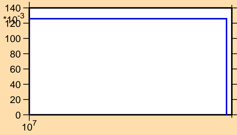
\sigma vs. E for ^{203}\text{Au}(n,3n)
