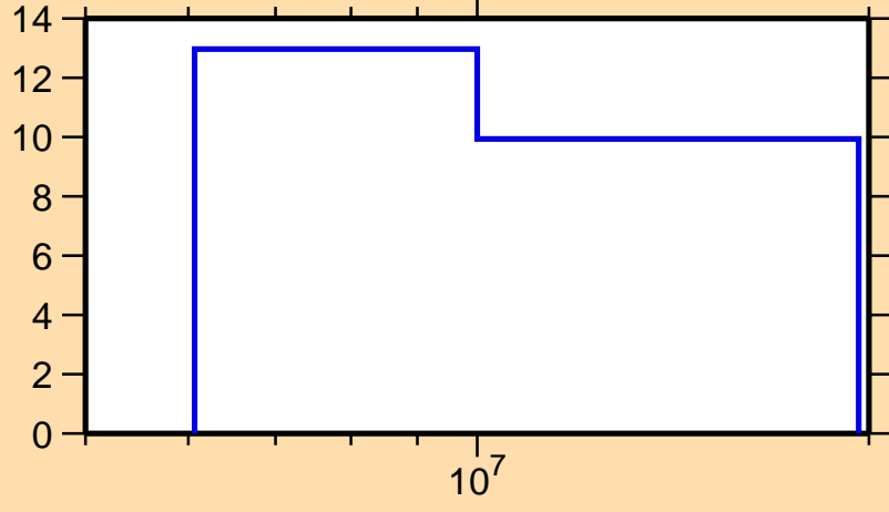
\Delta\sigma/\sigma vs. E for ^{203}\text{Au}(n,2n)
