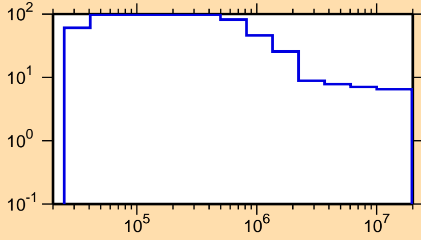
\Delta\sigma/\sigma vs. E for ^{203}\text{Au}(n,\text{nonel.})
