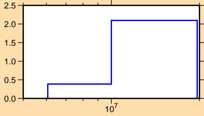
\sigma vs. E for ^{203}\text{Au}(n,2n)
