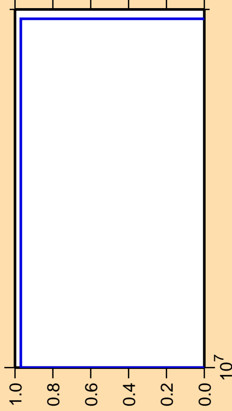
\Delta\sigma/\sigma vs. E for ^{203}\text{Au}(n,2np)
