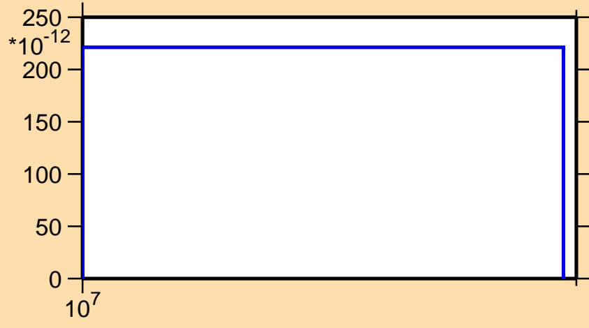
\sigma vs. E for ^{203}\text{Au}(n,nt)
