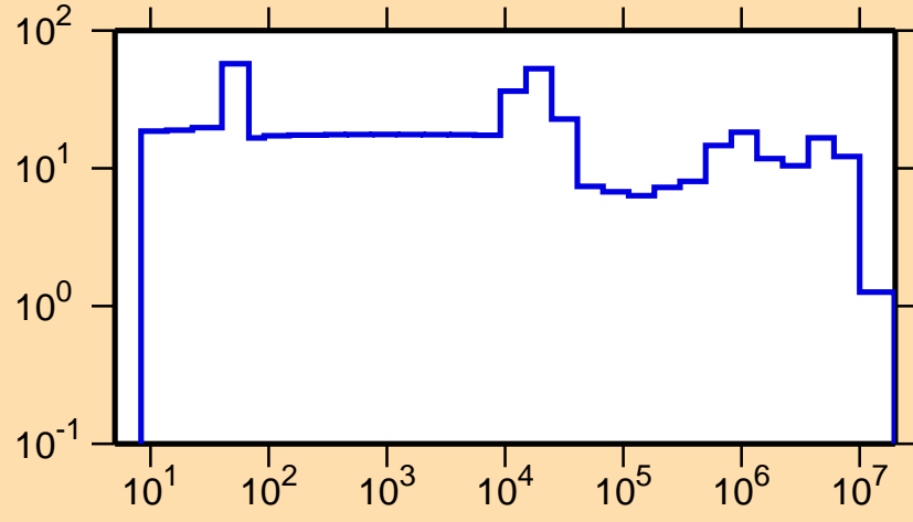
\Delta\sigma/\sigma vs. E for ^{203}\text{Au}(n,\text{el.})
