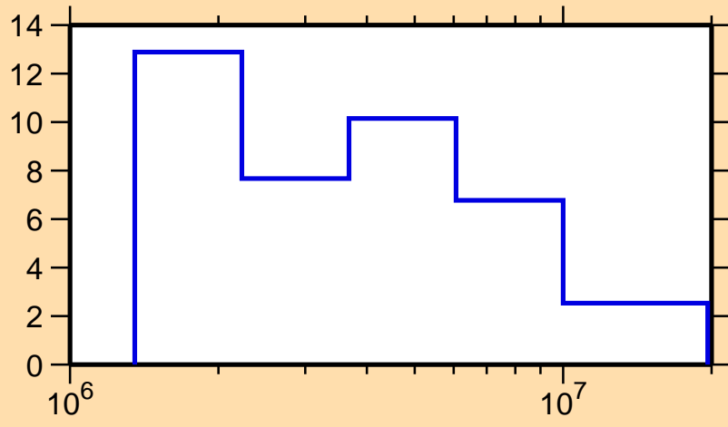
\Delta\sigma/\sigma vs. E for ^{203}\text{Au}(n,\text{tot.})
