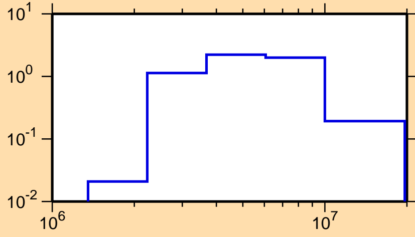
\sigma vs. E for ^{203}\text{Au}(n,n\text{cont.})
