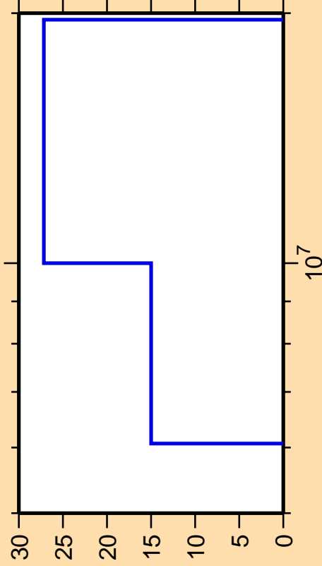
\Delta\sigma/\sigma vs. E for ^{203}\text{Au}(n,n\text{cont.})
