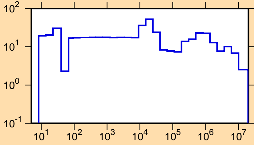
\Delta\sigma/\sigma vs. E for ^{203}\text{Au}(n,\text{tot.})
