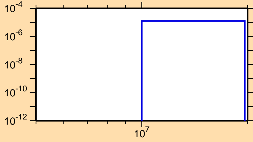
\sigma vs. E for ^{203}\text{Au}(n,np)
