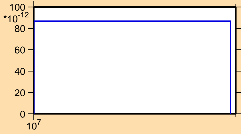
\sigma vs. E for ^{203}\text{Au}(n,\text{nd})
