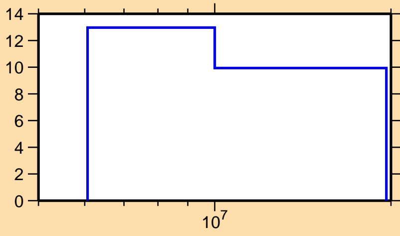
\Delta\sigma/\sigma vs. E for ^{203}\text{Au}(n,2n)
