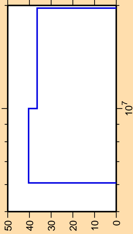
\Delta\sigma/\sigma vs. E for ^{203}\text{Au}(n,n_1)
