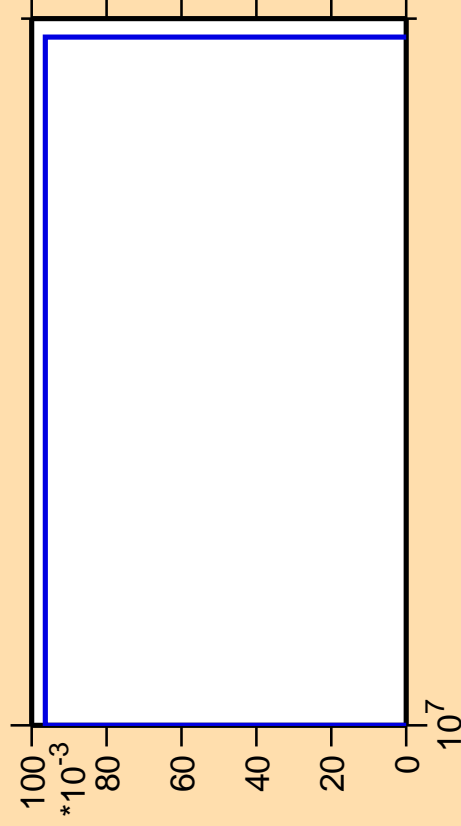
\Delta\sigma/\sigma vs. E for ^{203}\text{Au}(n,2n\alpha)
