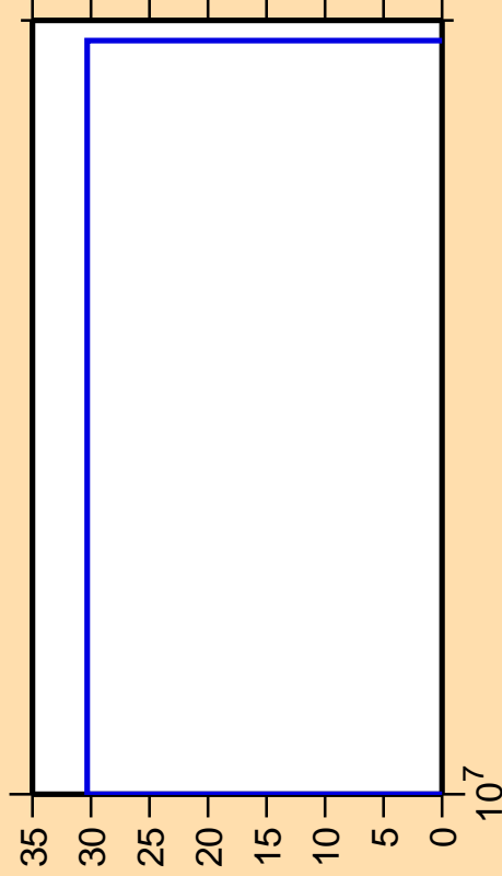
\Delta\sigma/\sigma vs. E for ^{203}\text{Au}(n,3n)
