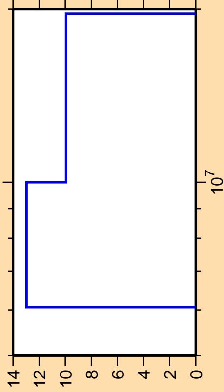
\Delta\sigma/\sigma vs. E for ^{203}\text{Au}(n,2n)
