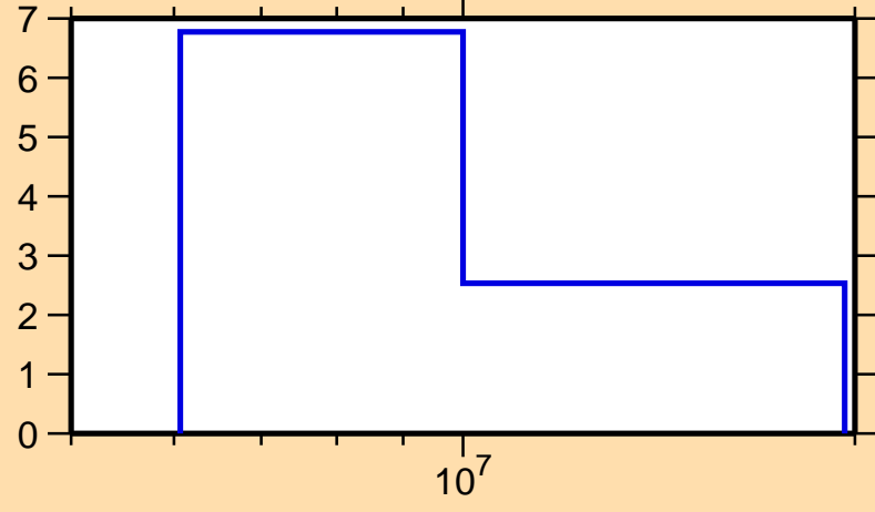
\Delta\sigma/\sigma vs. E for ^{203}\text{Au}(n,\text{tot.})
