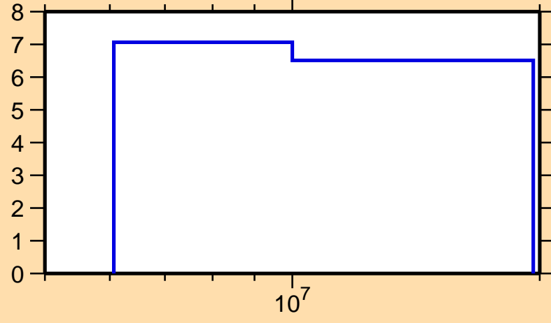
\Delta\sigma/\sigma vs. E for ^{203}\text{Au}(n,\text{nonel.})
