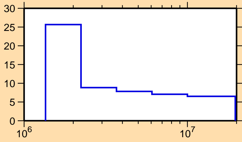
\Delta\sigma/\sigma vs. E for ^{203}\text{Au}(n,\text{nonel.})
