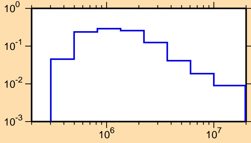
\sigma vs. E for ^{203}\text{Au}(n,n_2)
