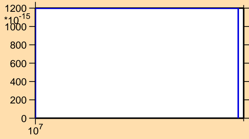
\sigma vs. E for ^{203}\text{Au}(n,2np)
